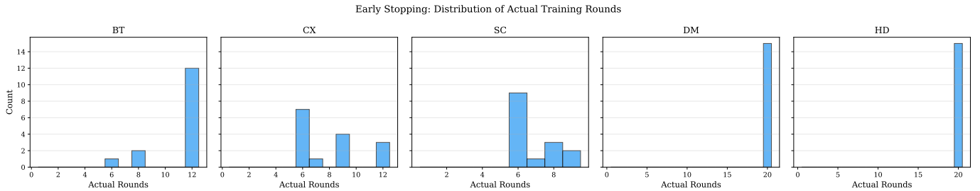
Fig. S-31. Early stopping analysis: actual rounds used vs. configured maximum. Most algorithms converge before the maximum round budget, demonstrating the effectiveness of patience-based early stopping.
