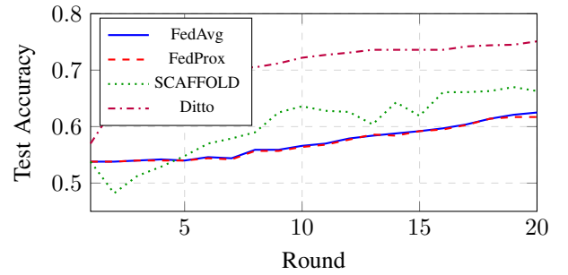
Fig. 2. Training convergence on Heart Disease UCI (4 hospitals, natural non-IID). Ditto converges faster and higher due to personalized local models.
