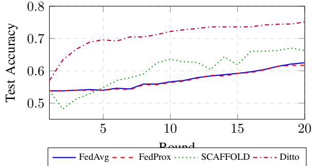
Fig. 2. Training convergence on Heart Disease UCI (4 hospitals, natural non-IID). Ditto converges faster and higher due to personalized local models.
