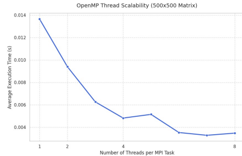
Fig. I.1: Average execution time as a function of threads per MPI task (500 × 500 matrix).
