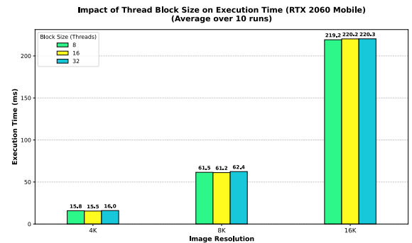
Fig. II.4: Impact of Thread Block Size on Execution Time on a RTX 2060 Mobile
