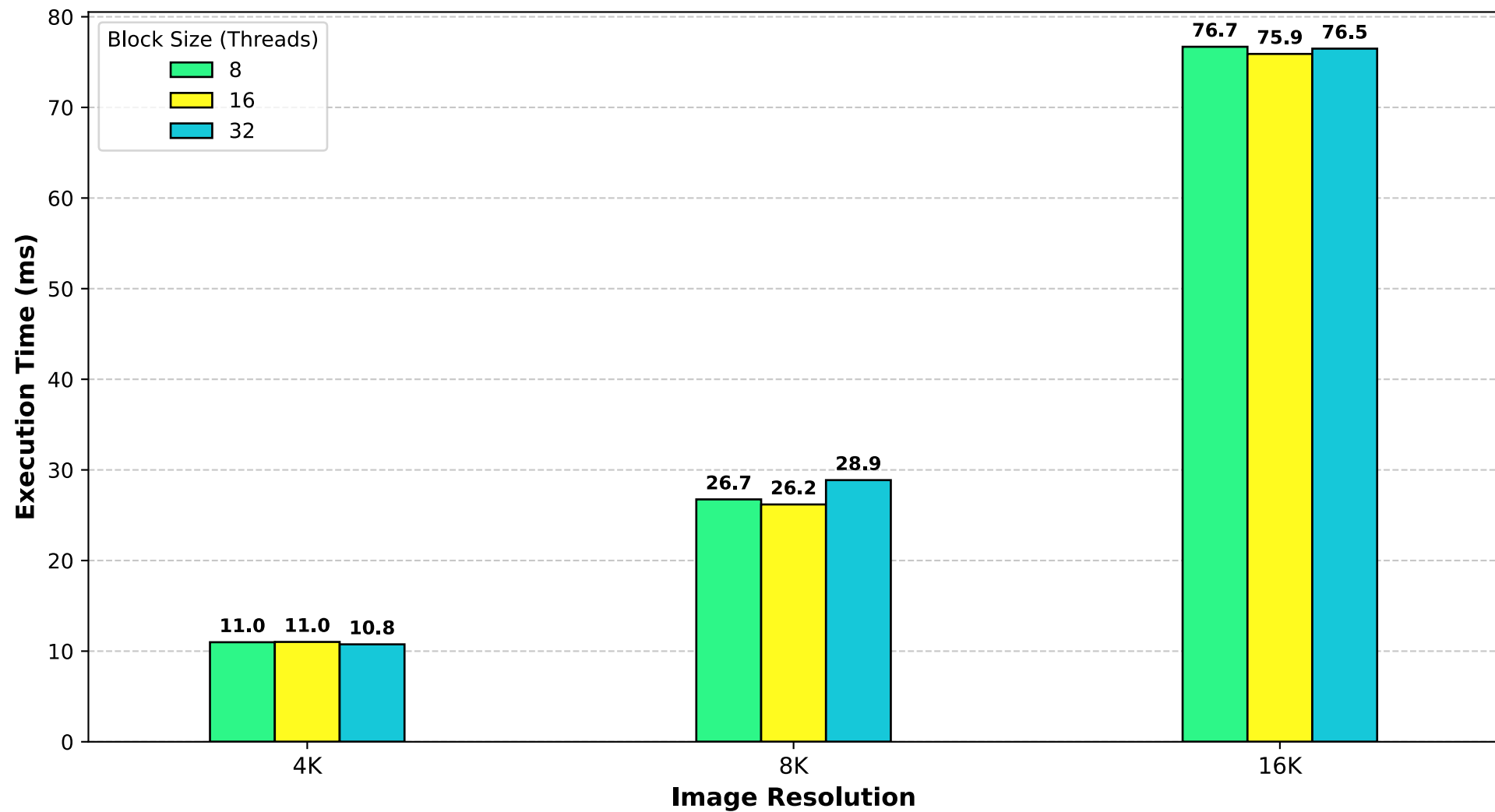
Impact of Thread Block Size on Execution Time (1 A100) (Average over 10 runs)
