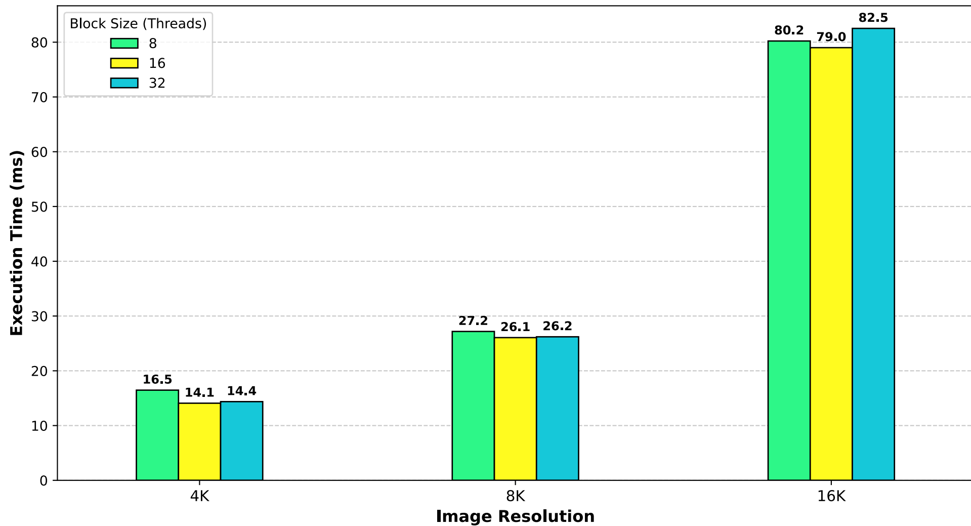
Impact of Thread Block Size on Execution Time (3 A100) (Average over 10 runs)
