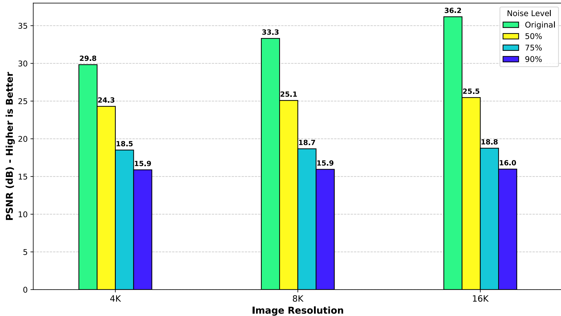
Filter Effectiveness: PSNR Degradation vs Impulse Noise (3 A100)
