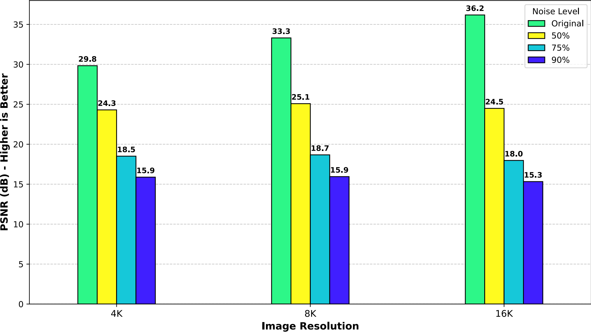
Filter Effectiveness: PSNR Degradation vs Impulse Noise (RTX 2060 Mobile)
