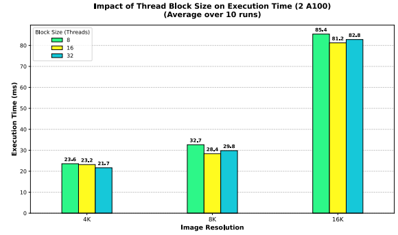
Fig. II.2: Impact of Thread Block Size on Execution Time on two NVIDIA A100
