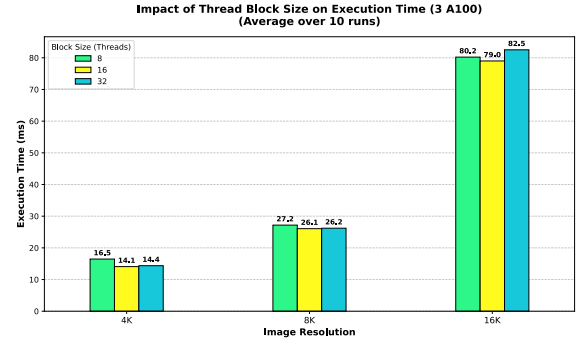
Fig. II.3: Impact of Thread Block Size on Execution Time on three NVIDIA A100
