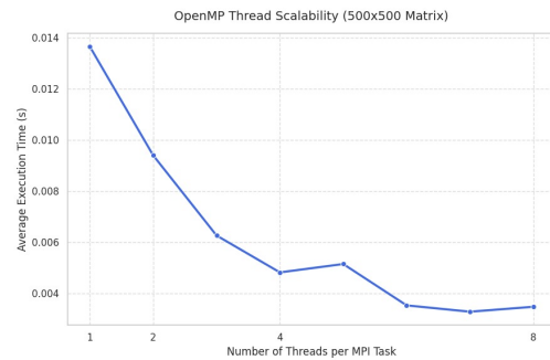
Fig. I.1: Average execution time as a function of threads per MPI task (500 × 500 matrix).
