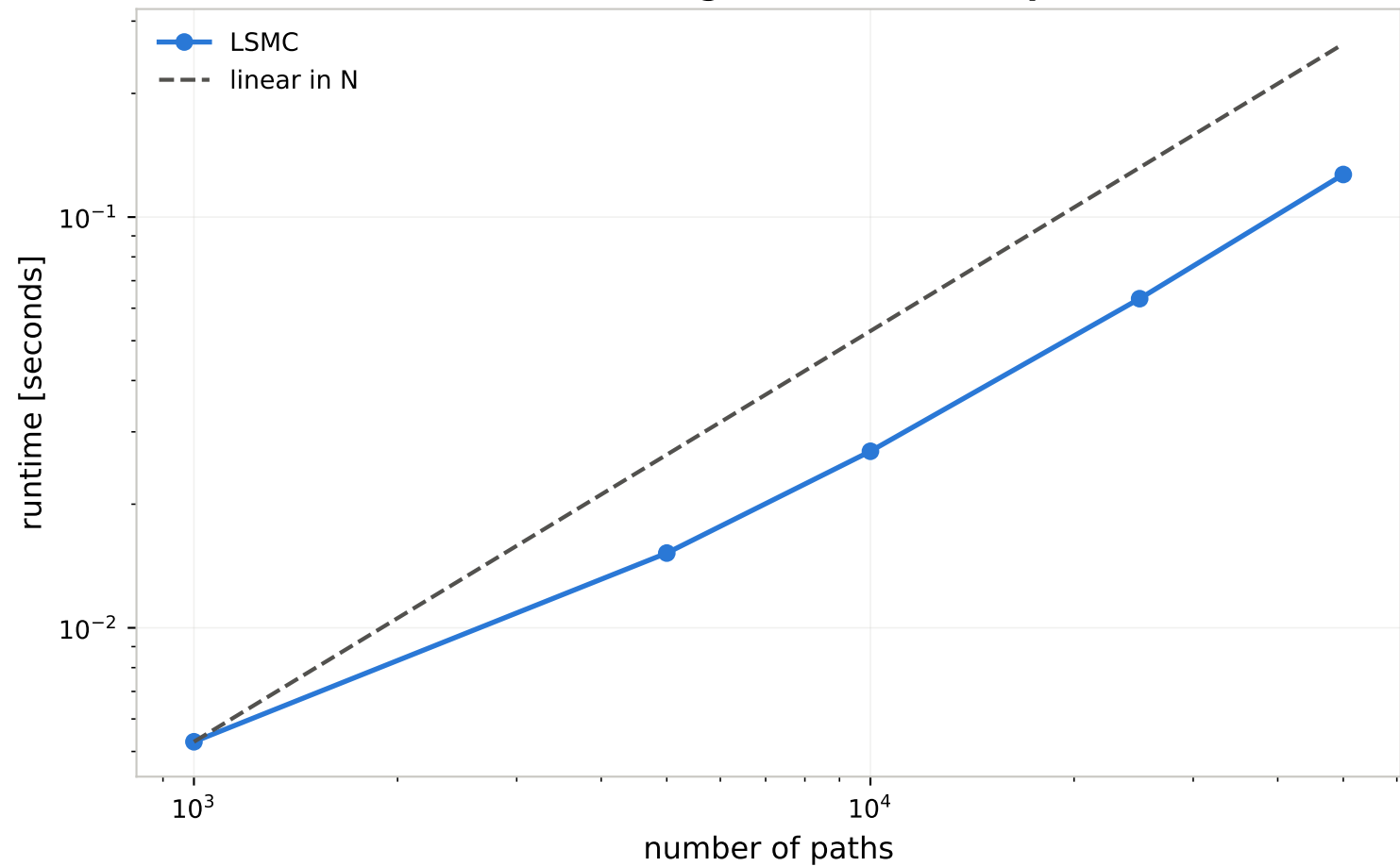
LSMC runtime against number of paths
