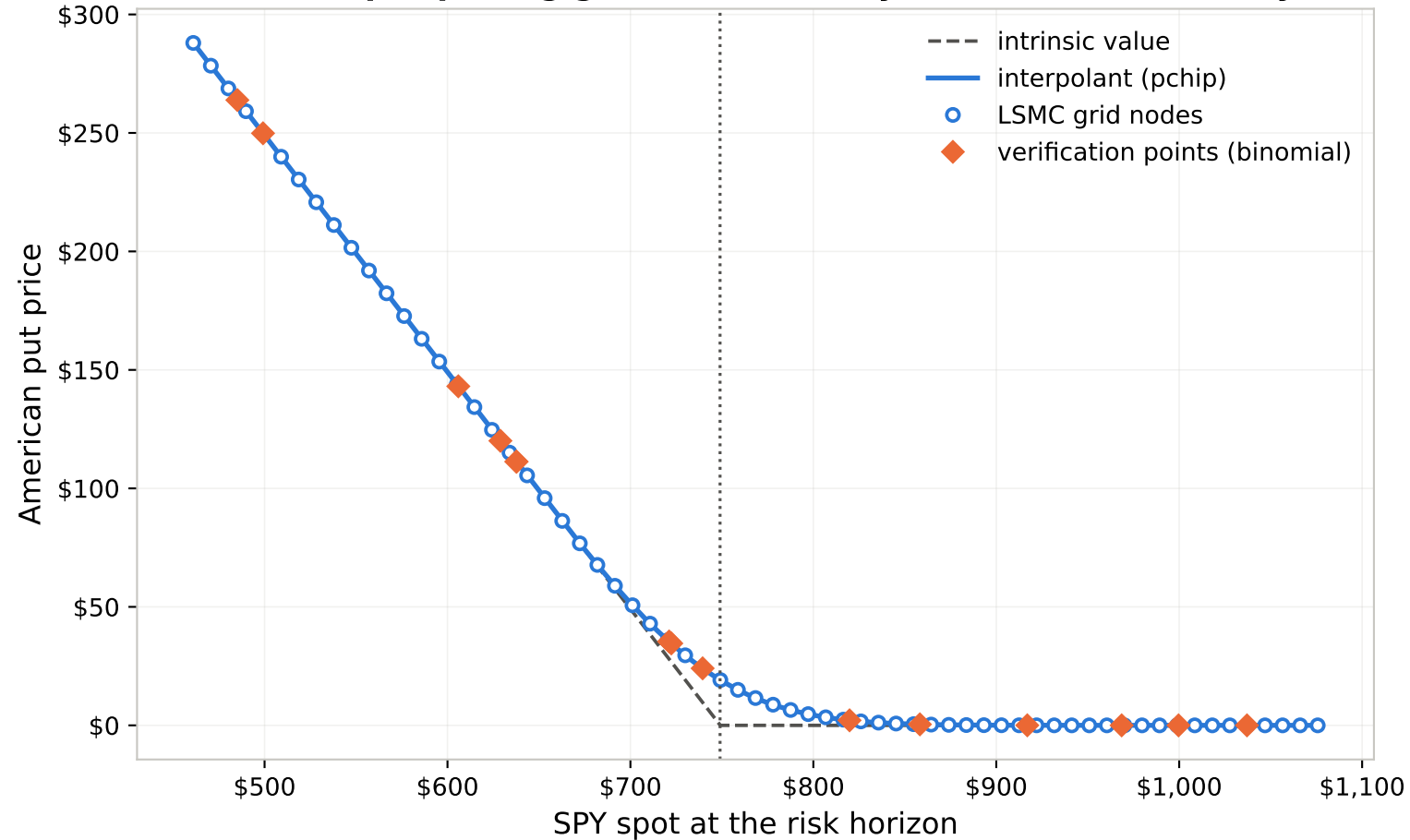
American put pricing grid at the 10-day horizon ( T = 0.1603 yr)
