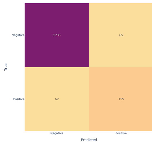
Figure 3: Confusion matrix for the Von-Heijne model
