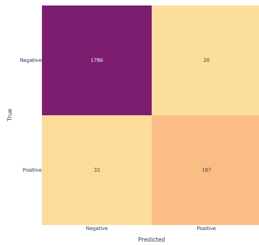
Figure 6: Confusion matrix for the SVM model
