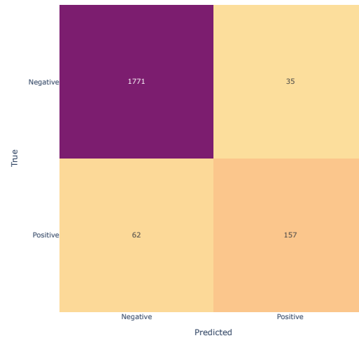
Figure 8: Confusion matrix for the reduced SVM model
