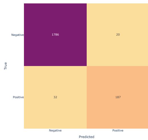
Figure 9: Confusion matrix for the SVM model
