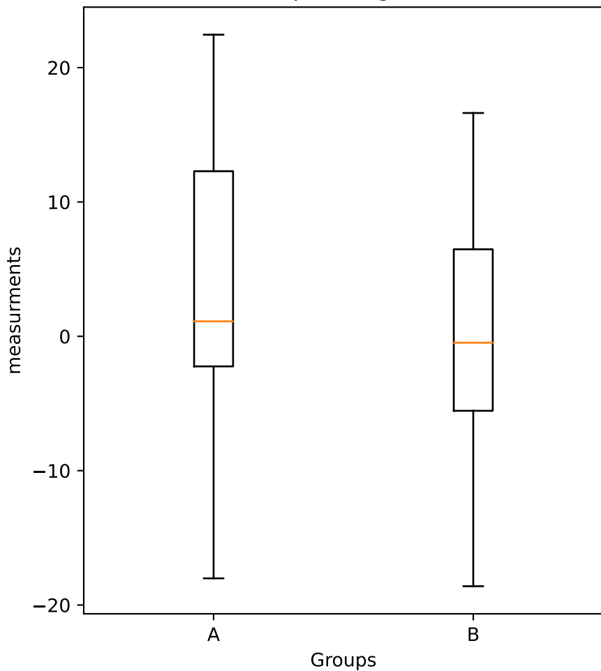
Boxplot diagram
