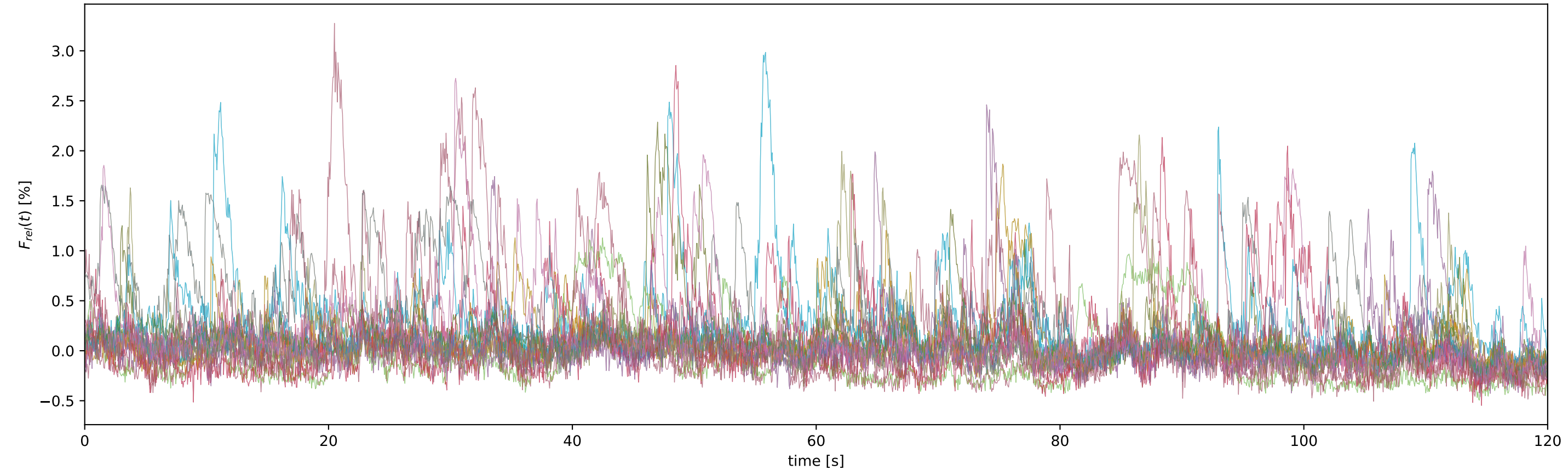
Relative fluorescence changes of Ca^{+2} signals
