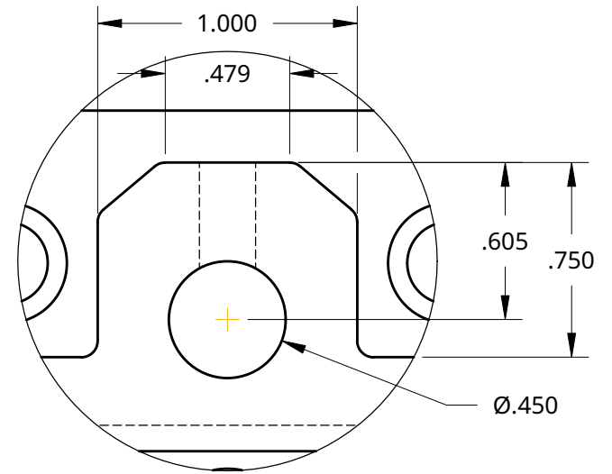
DETAIL A SCALE 3:2
