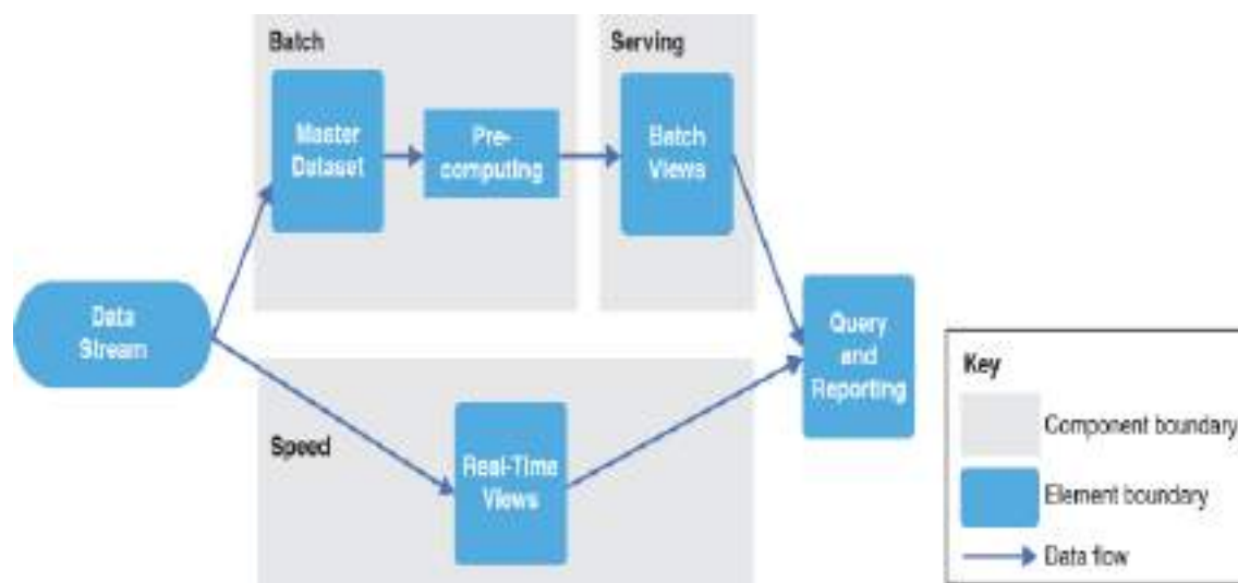
Figure 20.4 Example preliminary documentation
