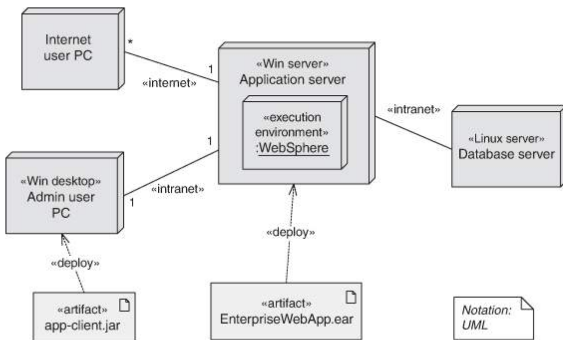
Figure 1.10 Deployment structure
