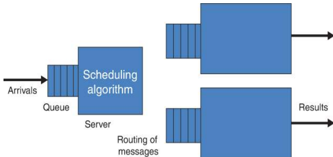
Figure 14.2 A generic queuing model
