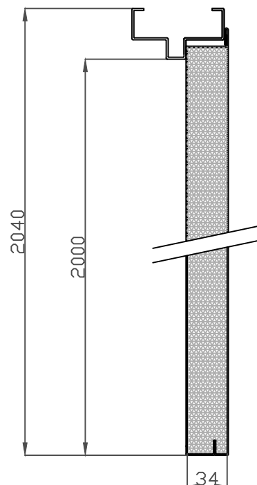
Corte vertical
