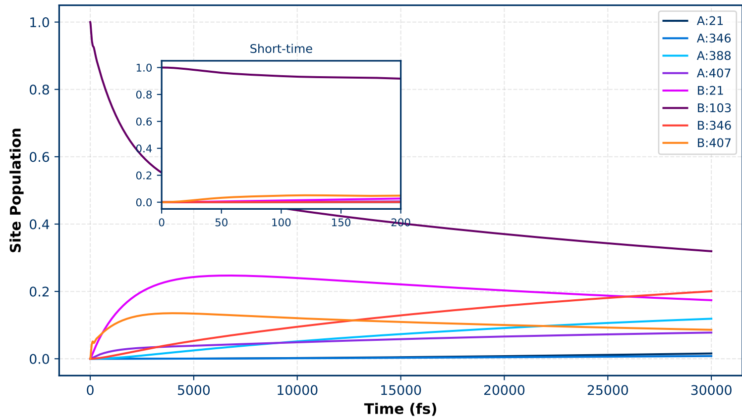
HEOM Benchmark (1JFF, NC=7, Nk=1)
