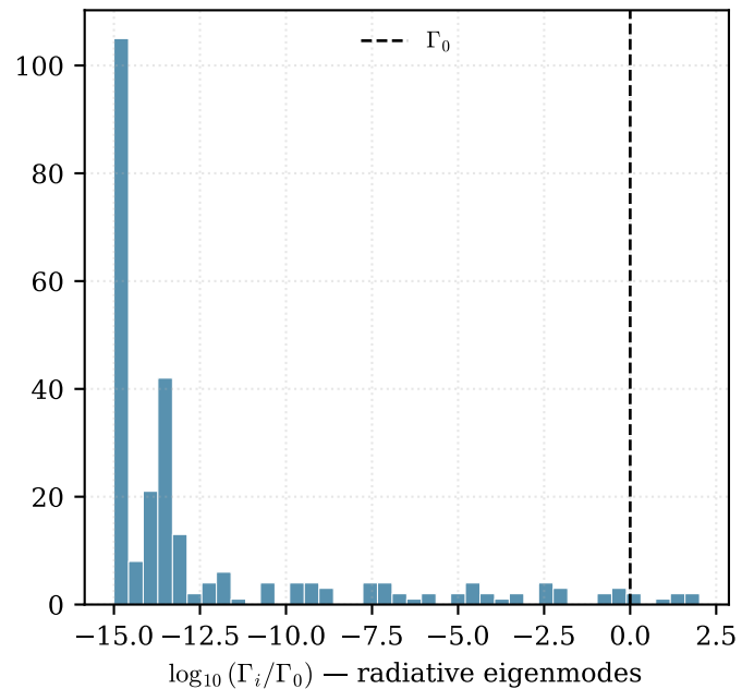
Radiative decay spectrum
