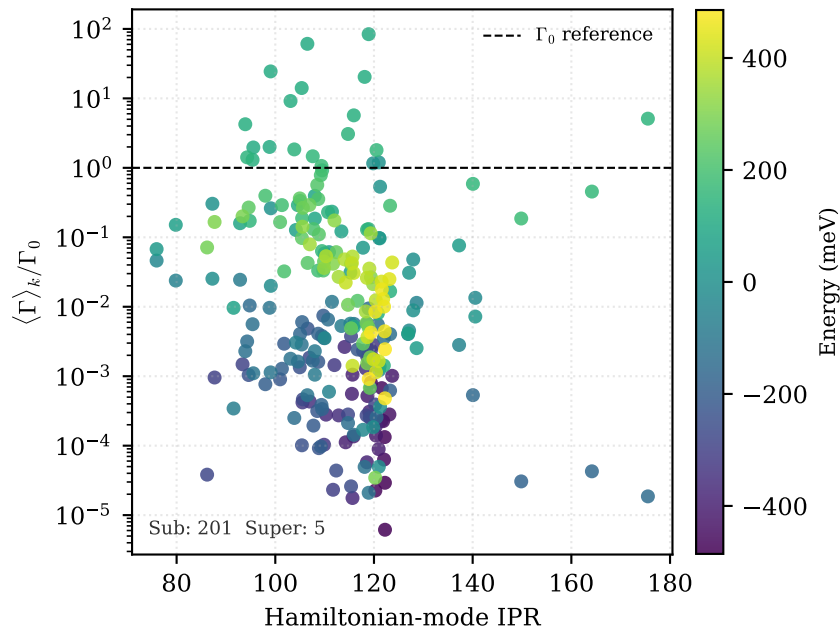
IPR vs radiative rate (colour = energy / meV)
