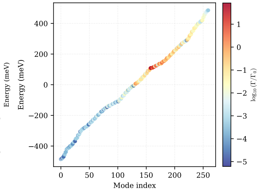
Excitonic spectrum (colour = \log_{10} \Gamma / \Gamma_0 )
