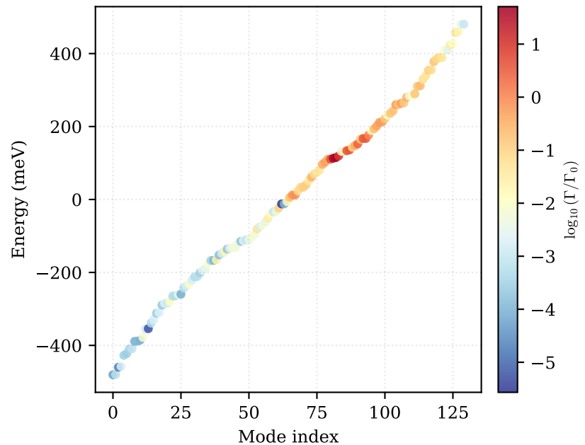
Excitonic spectrum (colour = \log_{10} \Gamma/\Gamma_0 )
