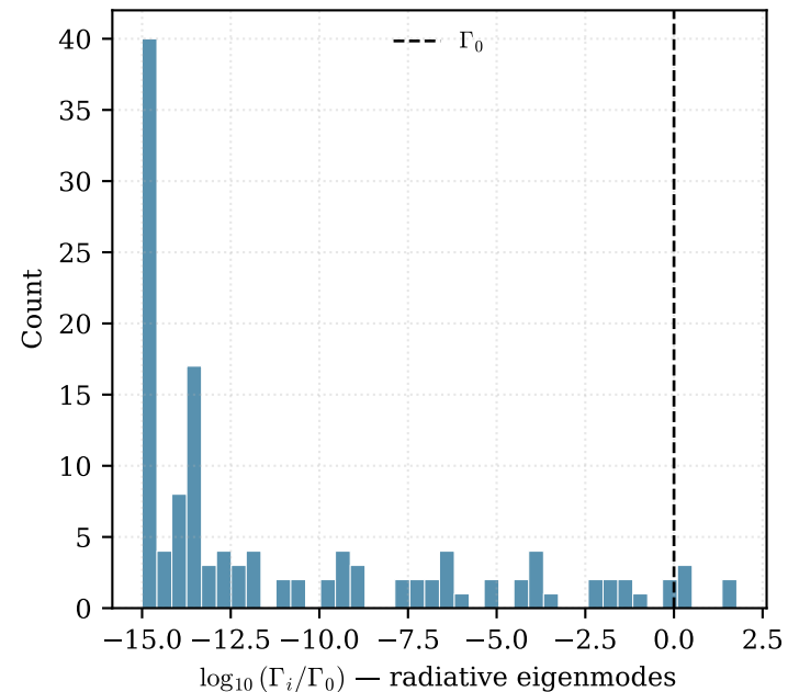
Radiative decay spectrum
