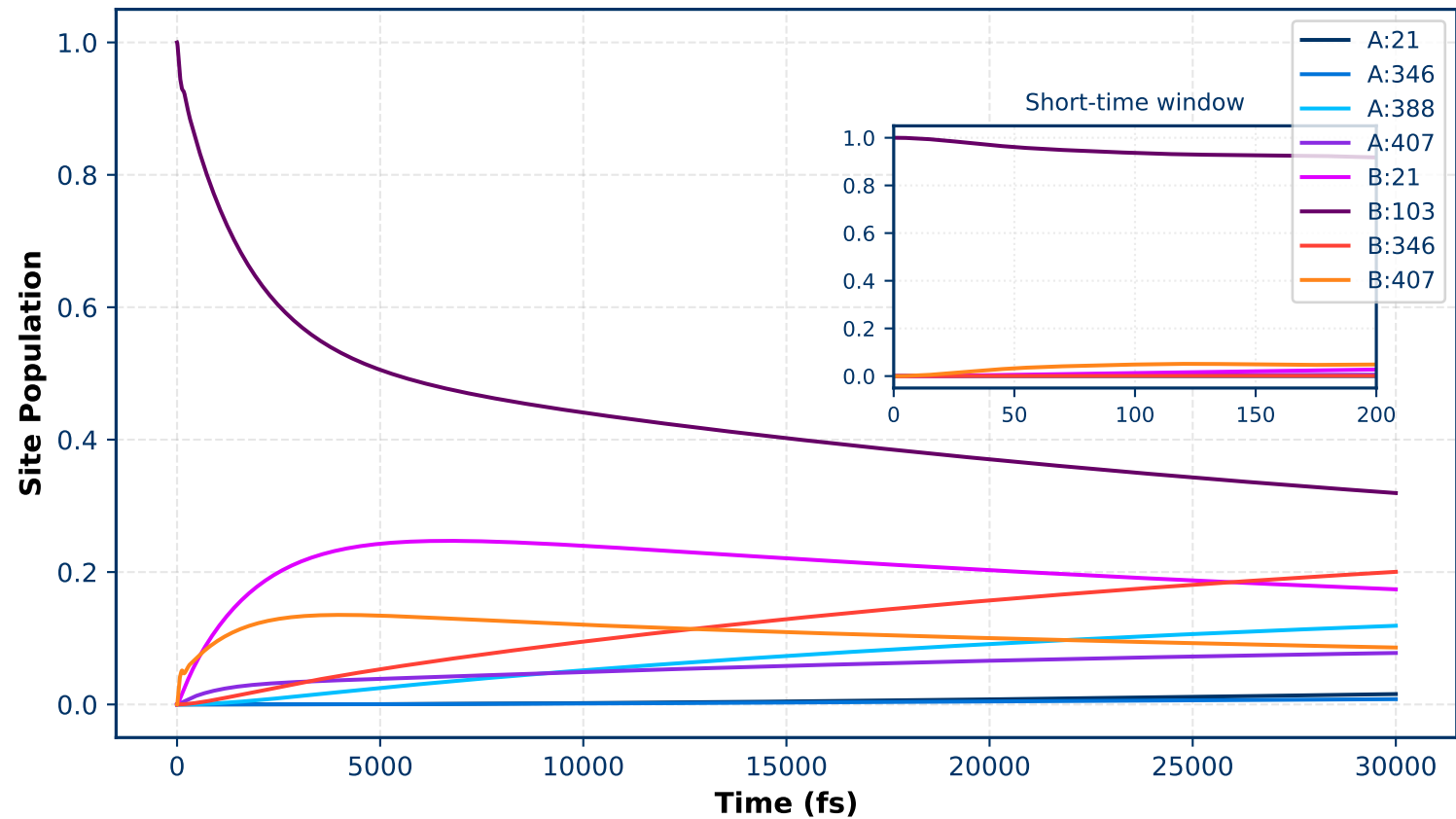
HEOM benchmark: 1JFF full (NC=7, Nk=1)
