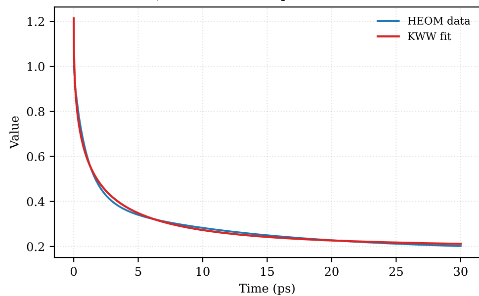
density_diagonal_purity \beta=0.436 , \tau=1.19 ps, R^2=0.993
