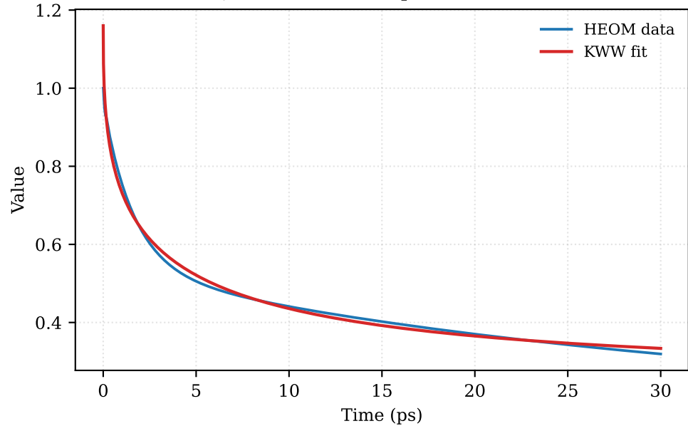
density_initial_site_population \beta=0.412 , \tau=2.81 ps, R^2=0.992
