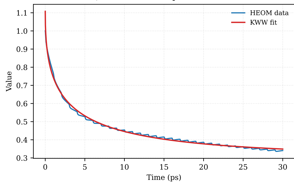
quantum_purity \beta=0.443 , \tau=1.17 ps, R^2=0.992
