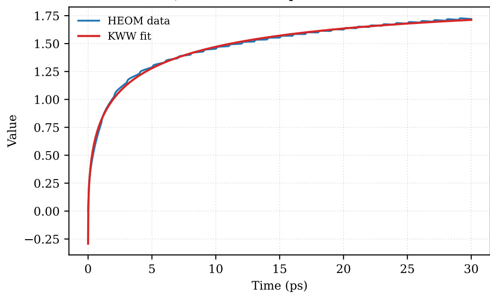
l1_coherence \beta=1.113 , \tau=1.78 ps, R^2=0.959
