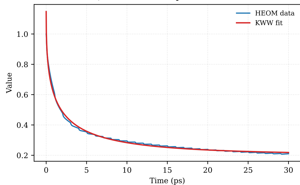
initial_site_population \beta=0.462 , \tau=3.03 ps, R^2=0.994
