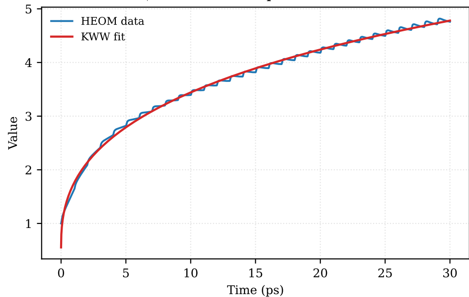
population_shannon_entropy \beta=0.370 , \tau=2.7 ps, R^2=0.997
