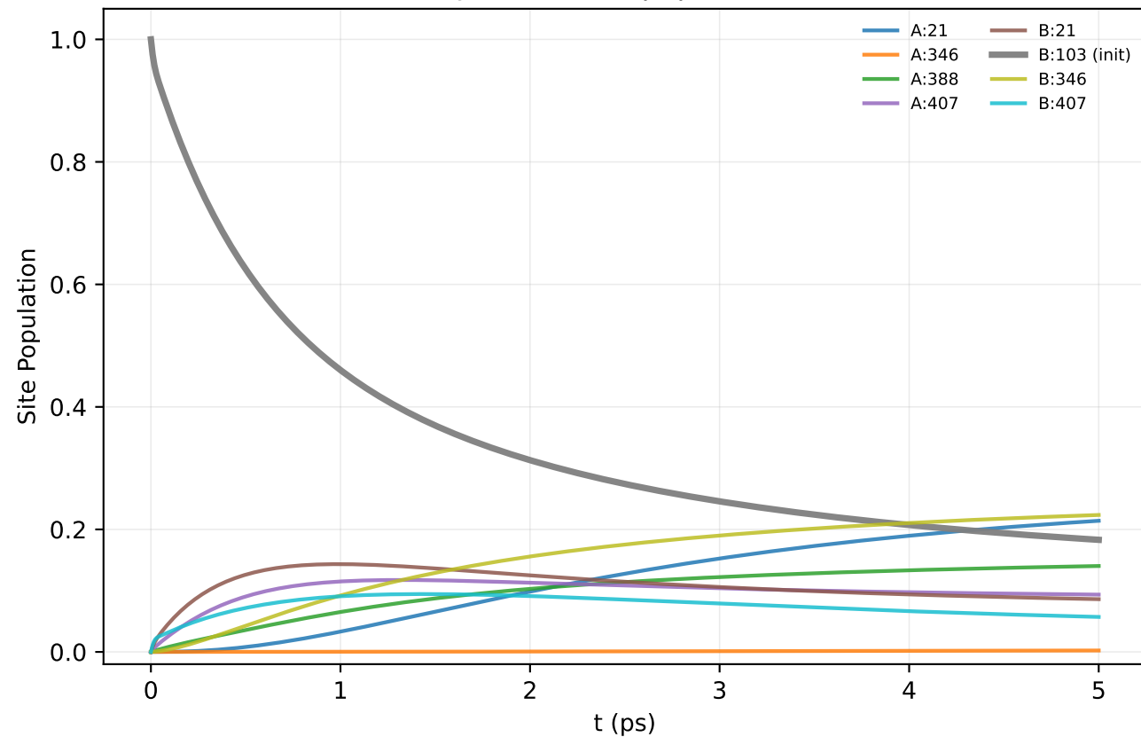
1JFF: Redfield populations
