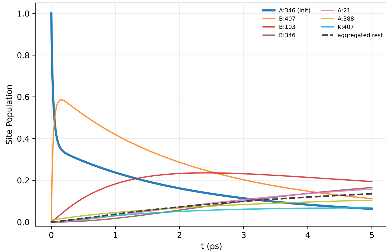
6DPU: Redfield populations
