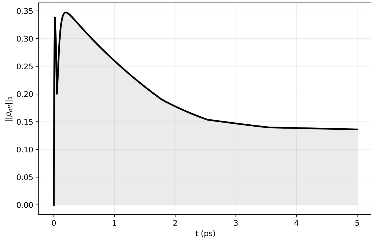
6DPU: Total L1 coherence
