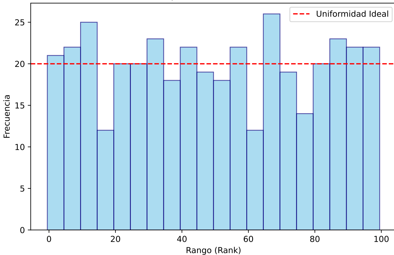
SBC Rank Histogram: Nested Sampling Engine (p-value = 0.8009)
