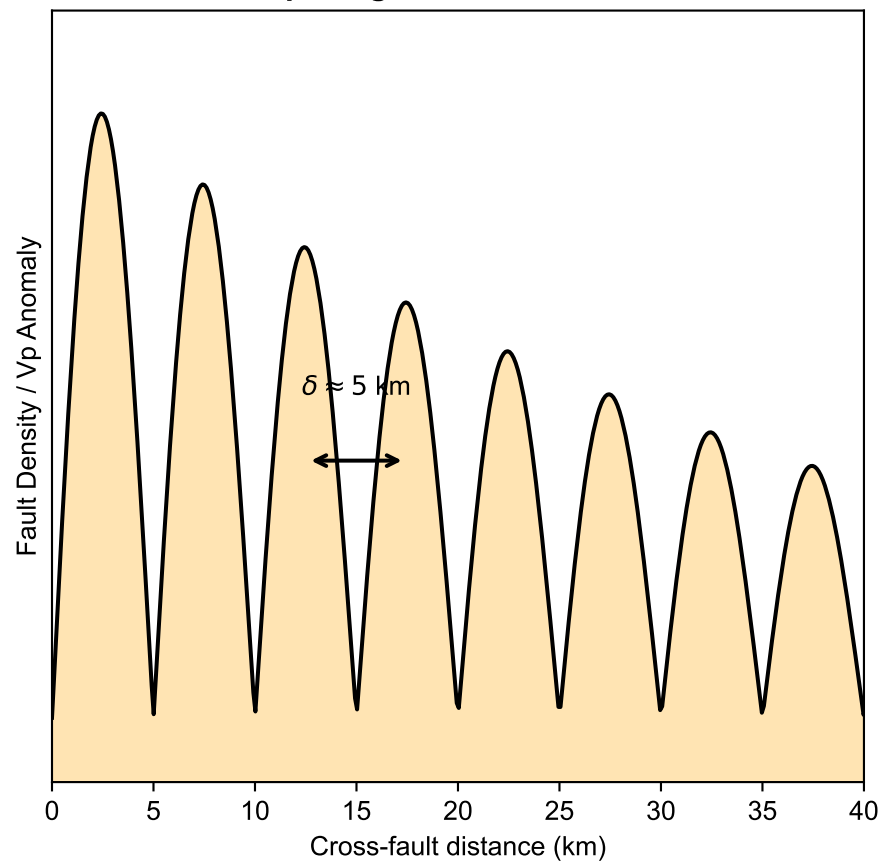
B. Fault Zone Spacing
