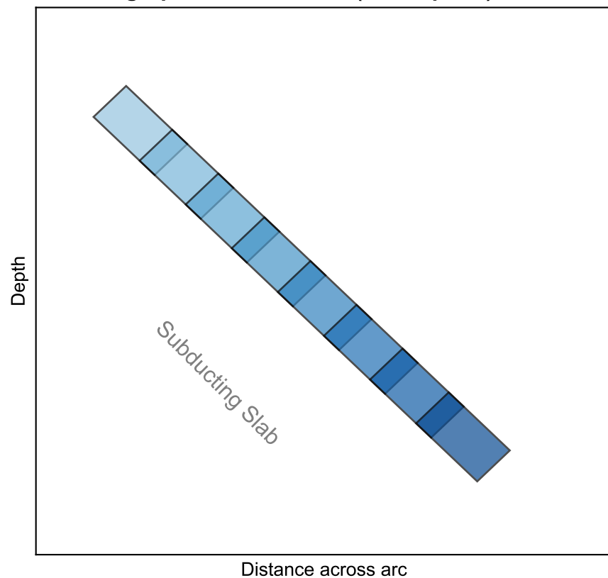
A. Tomographic Fault Blocks (Conceptual)
