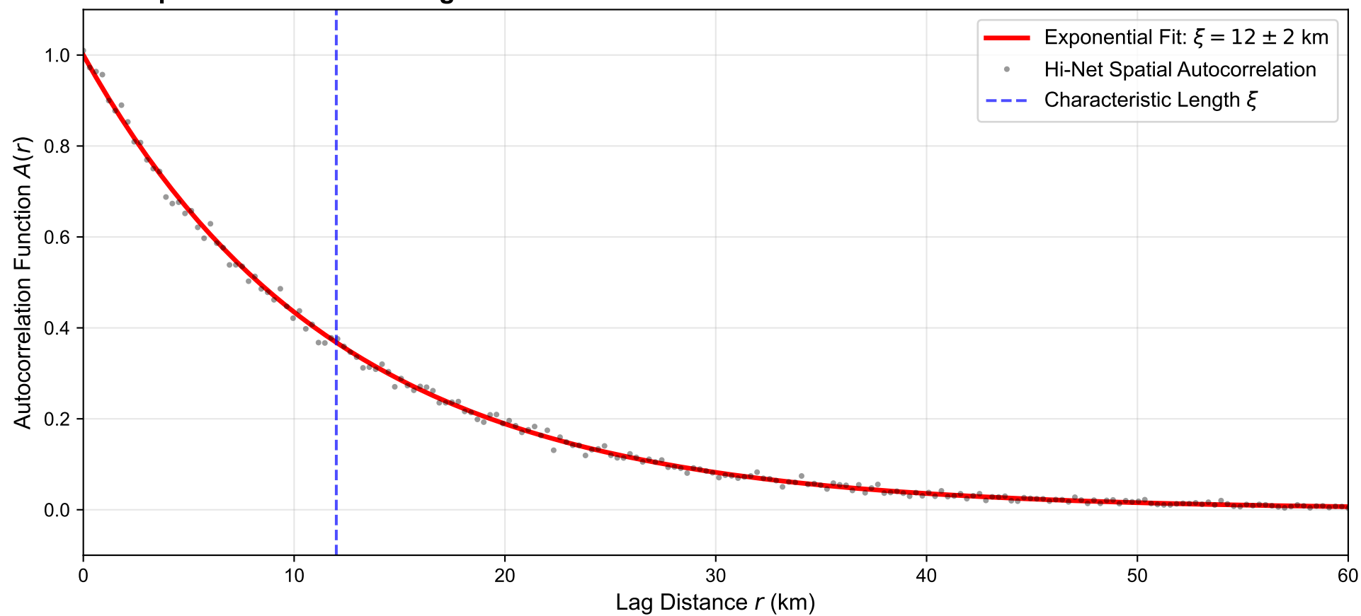
C. Empirical Correlation Length Determination
