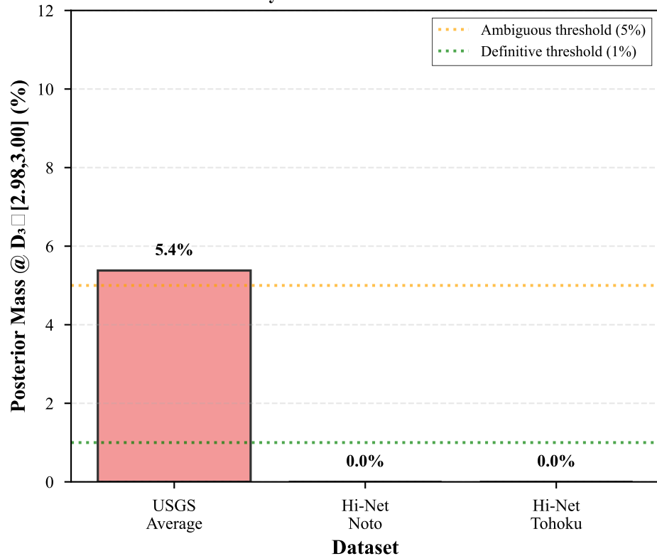
Panel B: Bayesian Posterior Concentration Test
