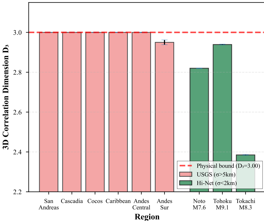
Panel A: D_3 Saturation @ 3.00 (USGS) vs Genuine (Hi-Net)
