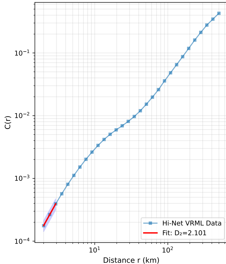
Hi-Net VRML: Real Data Defined D_2=2.10 ( r < 3 km)
