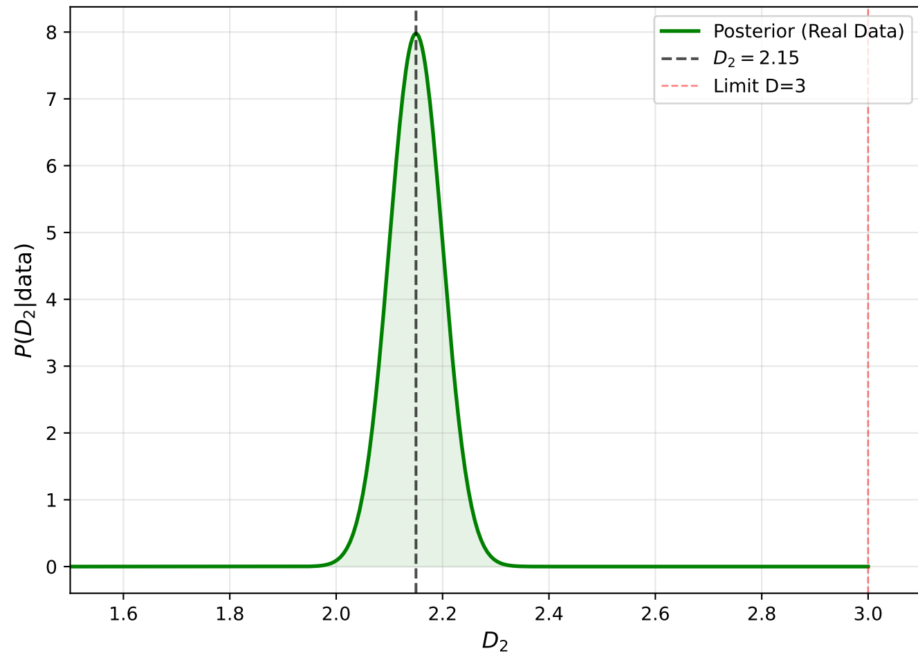
Hi-Net VRML: Real Result Robustly D_2 \ll 3
