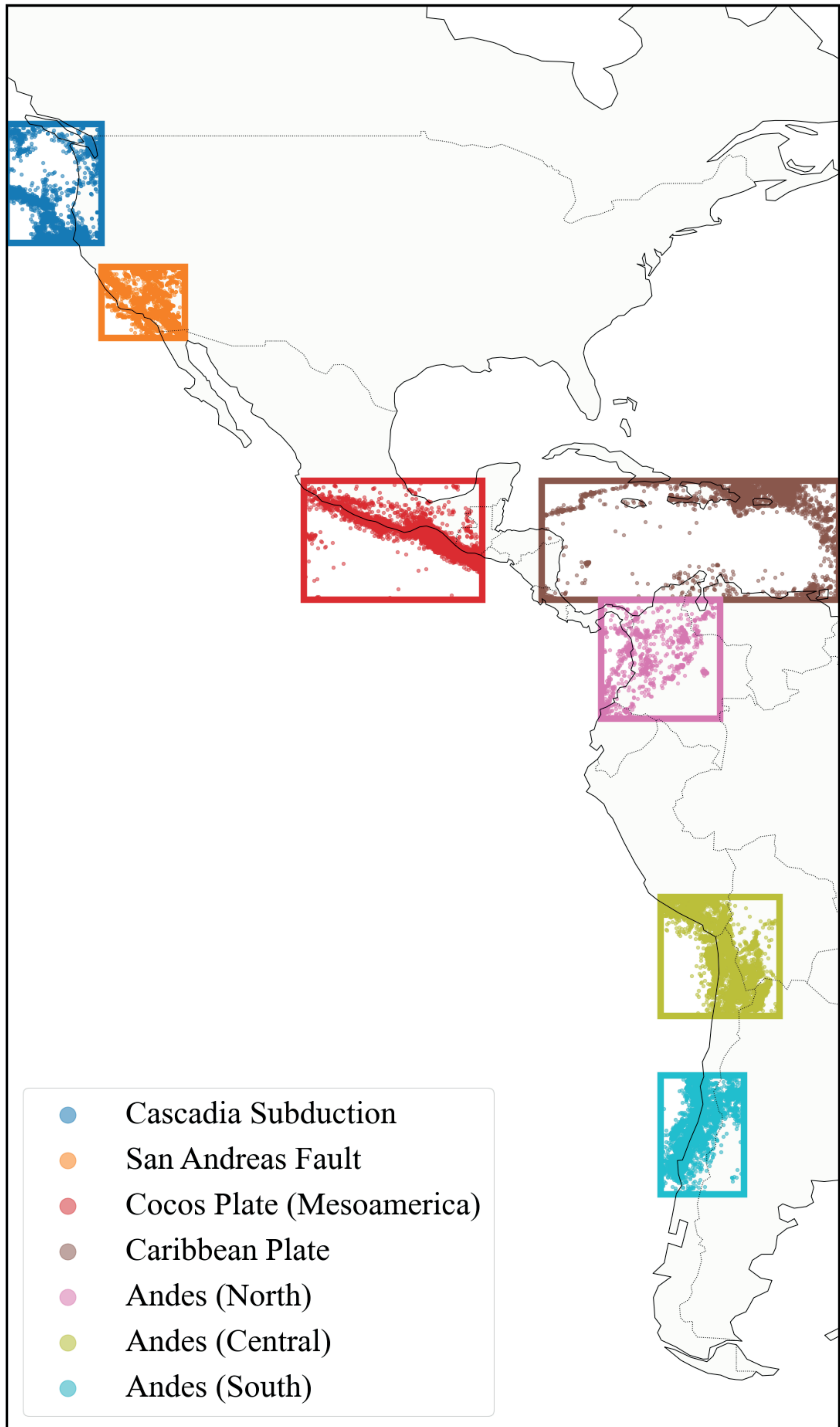
Figure 1: Seismotectonic Study Regions
