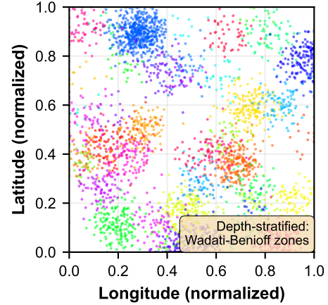
(C) Andes Central (Peru-Chile) 47 communities
