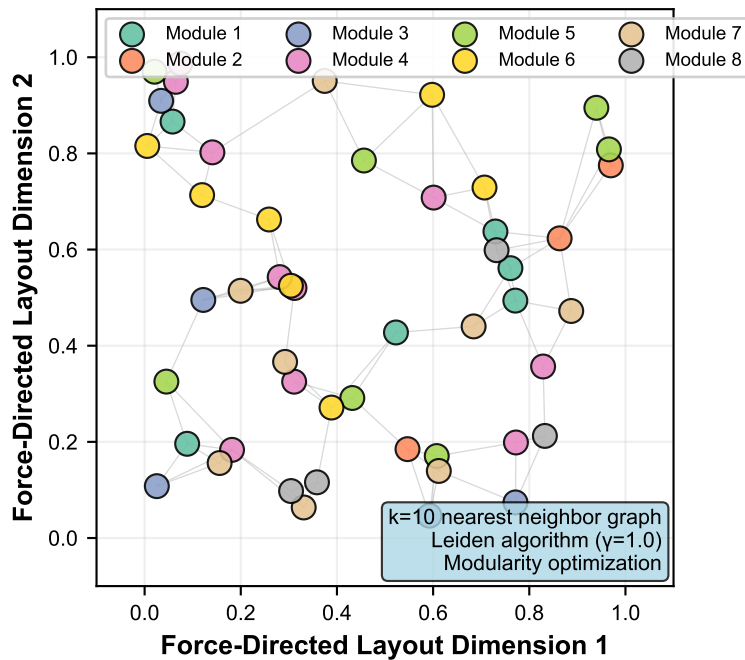
(D) Network Visualization: Dense Intra-Community / Sparse Inter-Community Connections
