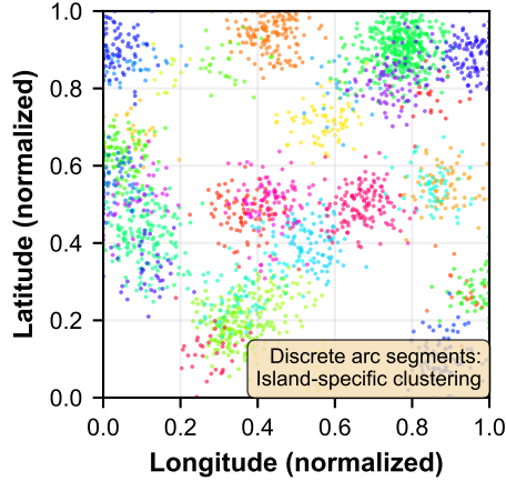
(B) Caribbean Plate (Lesser Antilles) 39 communities
