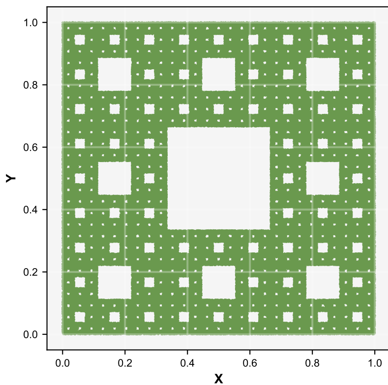
(C) Sierpiński Carpet: D_2 = 1.91 \pm 0.03
