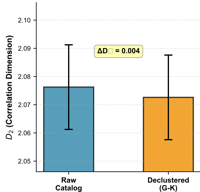
(A) San Andreas Fault
