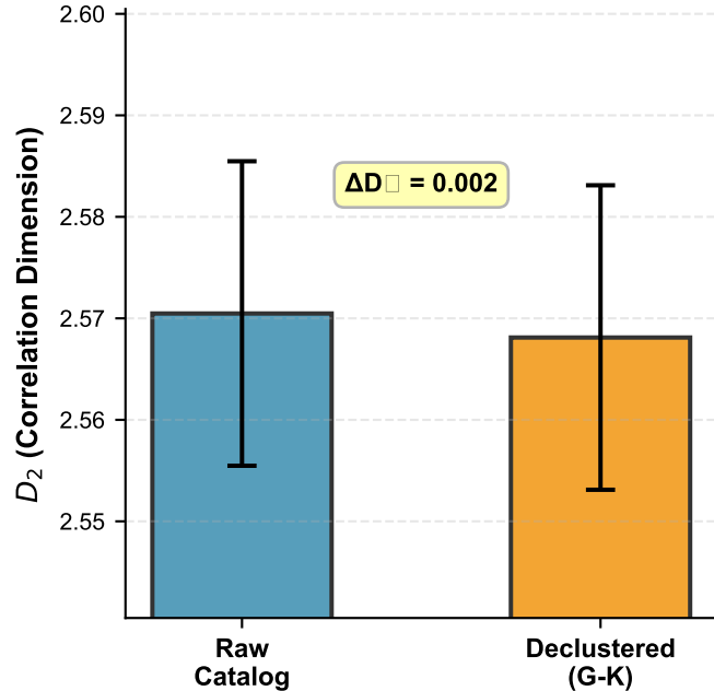
(C) Cocos Plate
