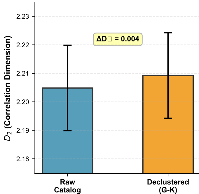
(B) Cascadia Subduction
