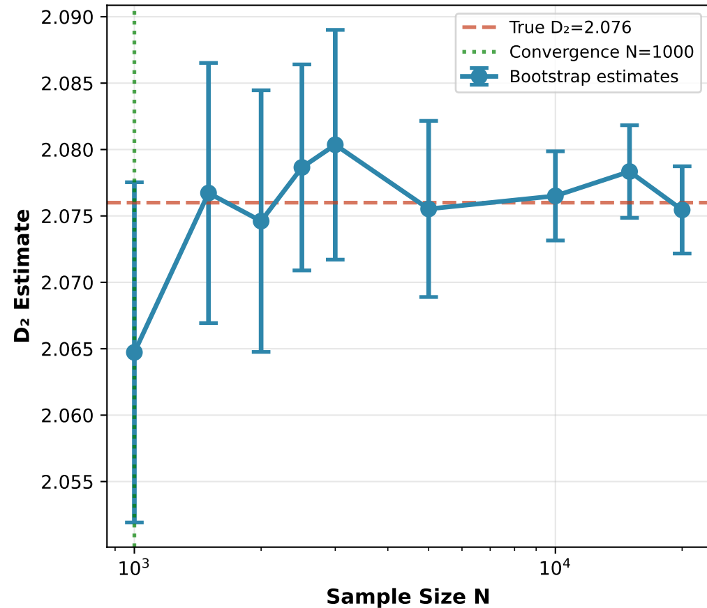
(A) D 2 Convergence vs Sample Size
