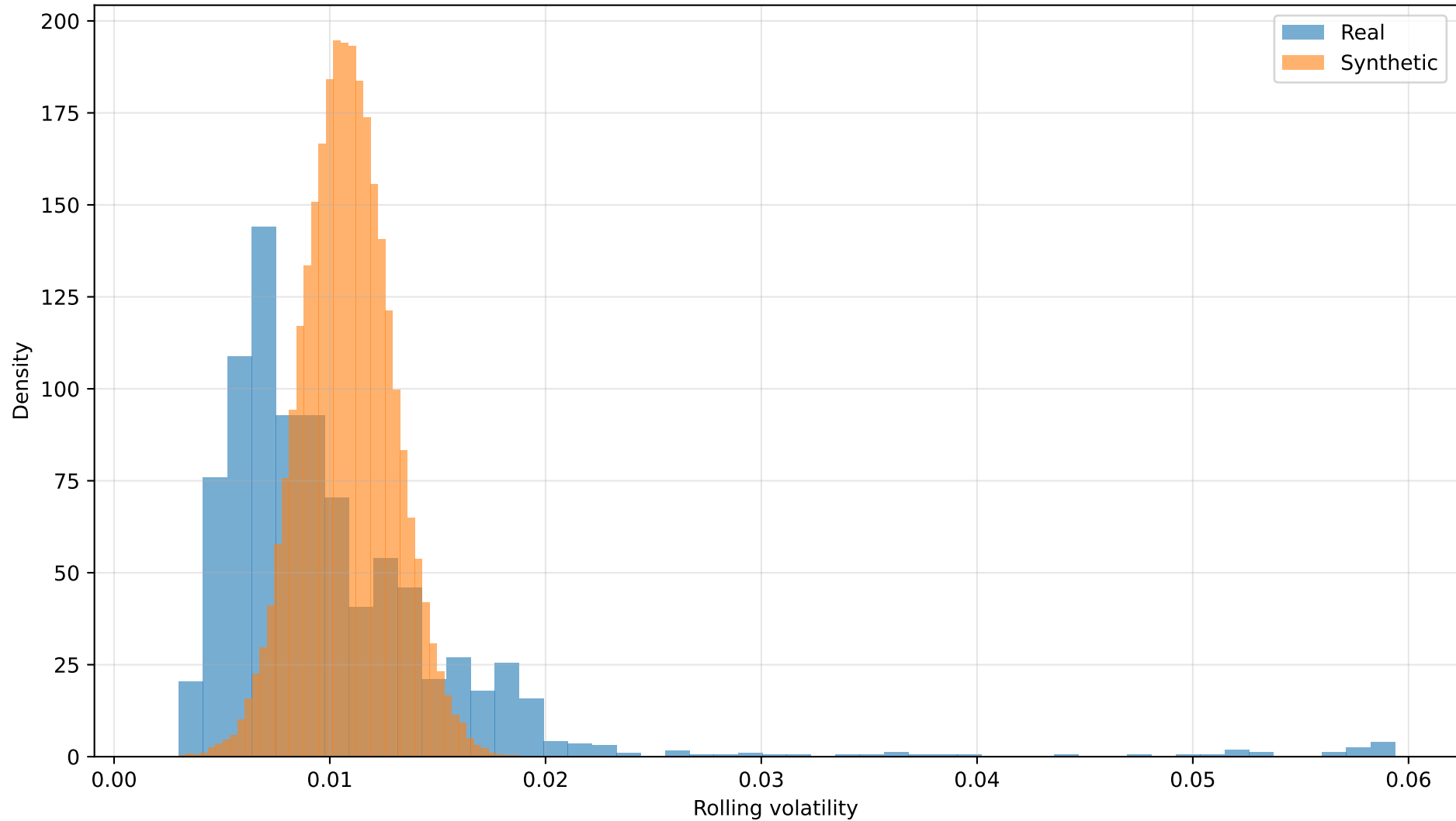
Rolling Volatility (20 steps): Real vs Synthetic
