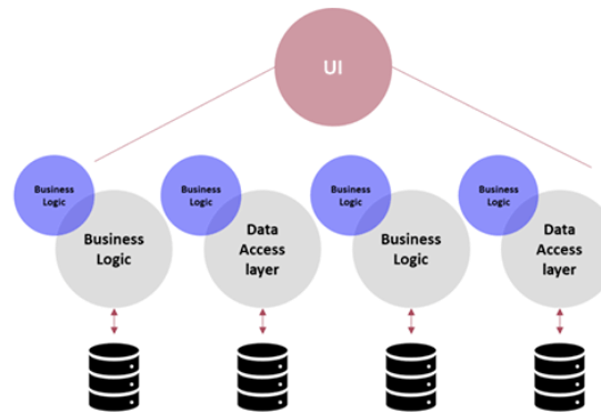
MICROSERVICE ARCHITECTURE
