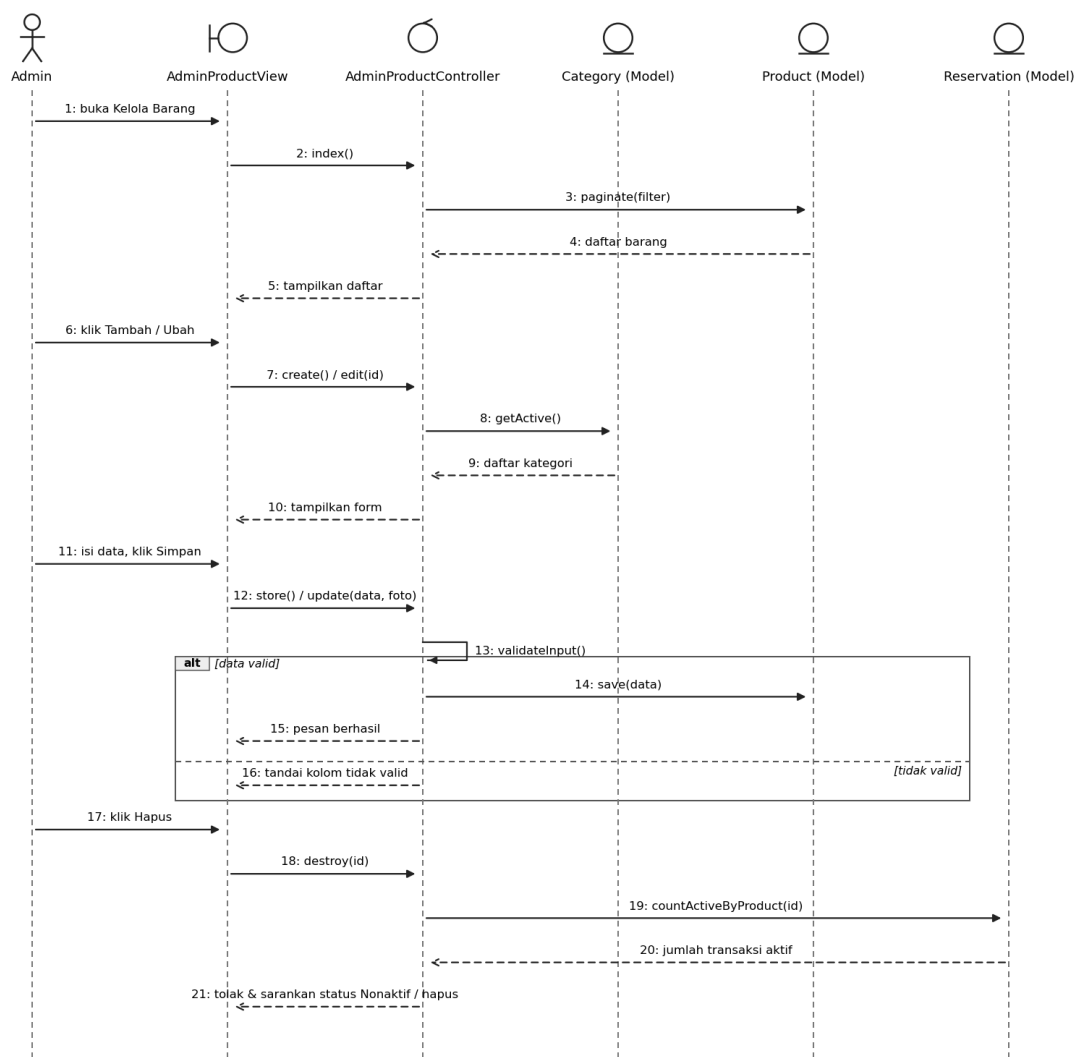
Gambar 3.32 Sequence diagram #10 Mengelola Barang
