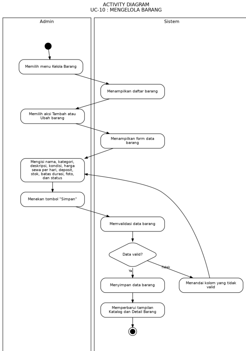
Gambar 3.33 Activity diagram #10 Mengelola Barang
