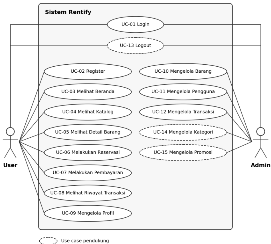
Gambar 3.1 Use case diagram Rentify
