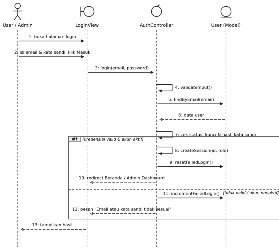
Gambar 3.3 Sequence diagram #1 Masuk Akun
