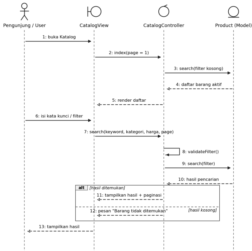
Gambar 3.12 Sequence diagram #4 Melihat Katalog
