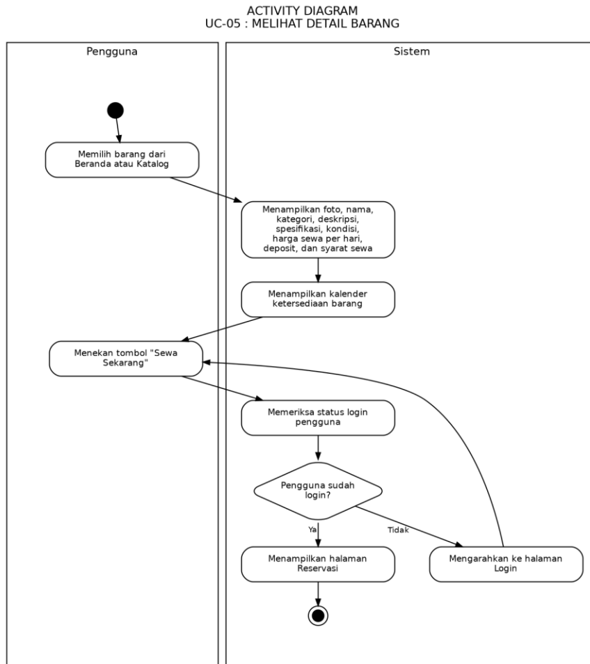
Gambar 3.16 Activity diagram #5 Melihat Detail Barang
