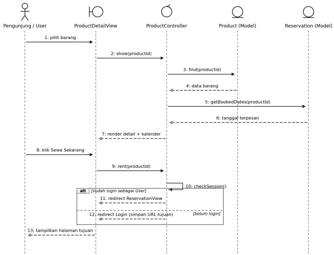
Gambar 3.15 Sequence diagram #5 Melihat Detail Barang
