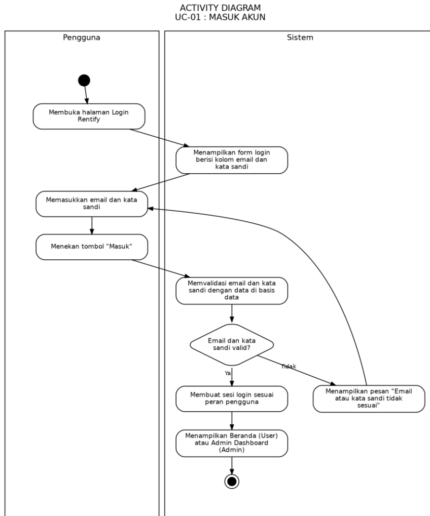
Gambar 3.4 Activity diagram #1 Masuk Akun
