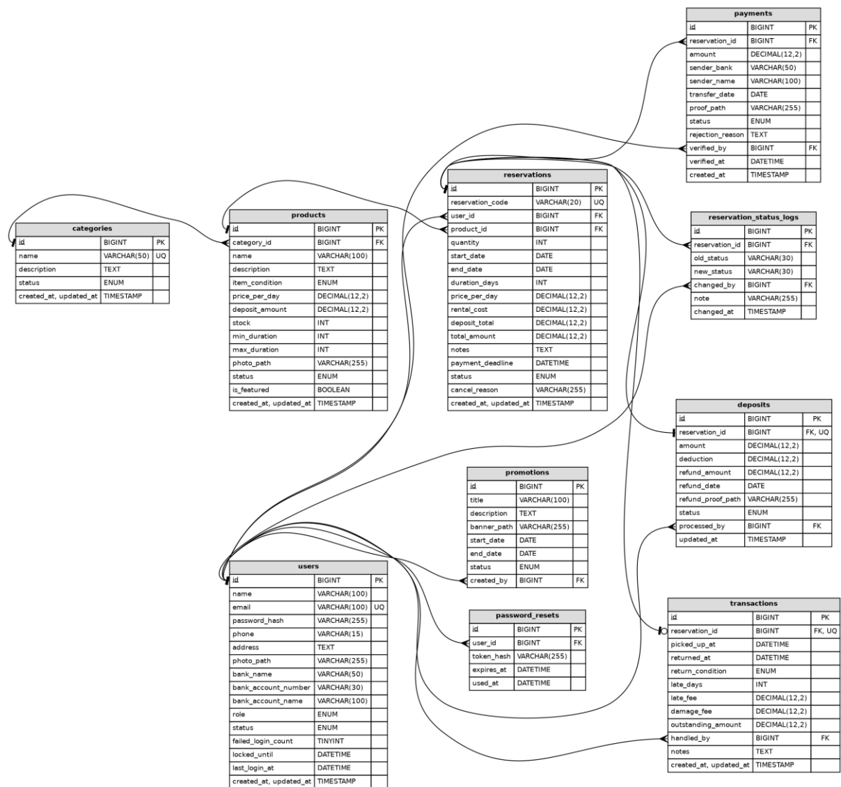
Gambar 3.43 Entity Relationship Diagram (ERD) Rentify
