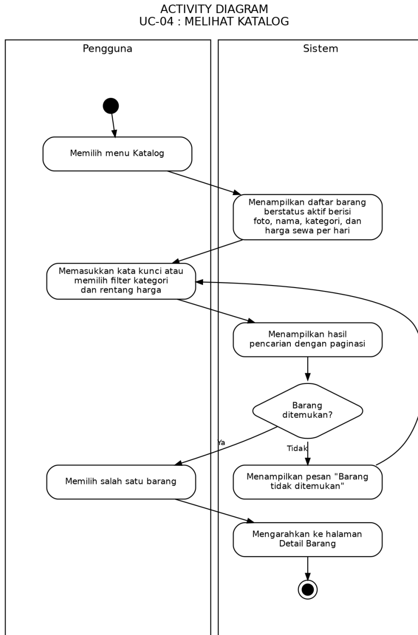
Gambar 3.13 Activity diagram #4 Melihat Katalog
