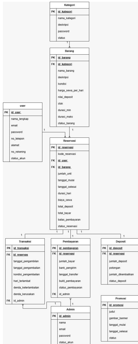
Gambar B.1 Entity Relationship Diagram Rentify
