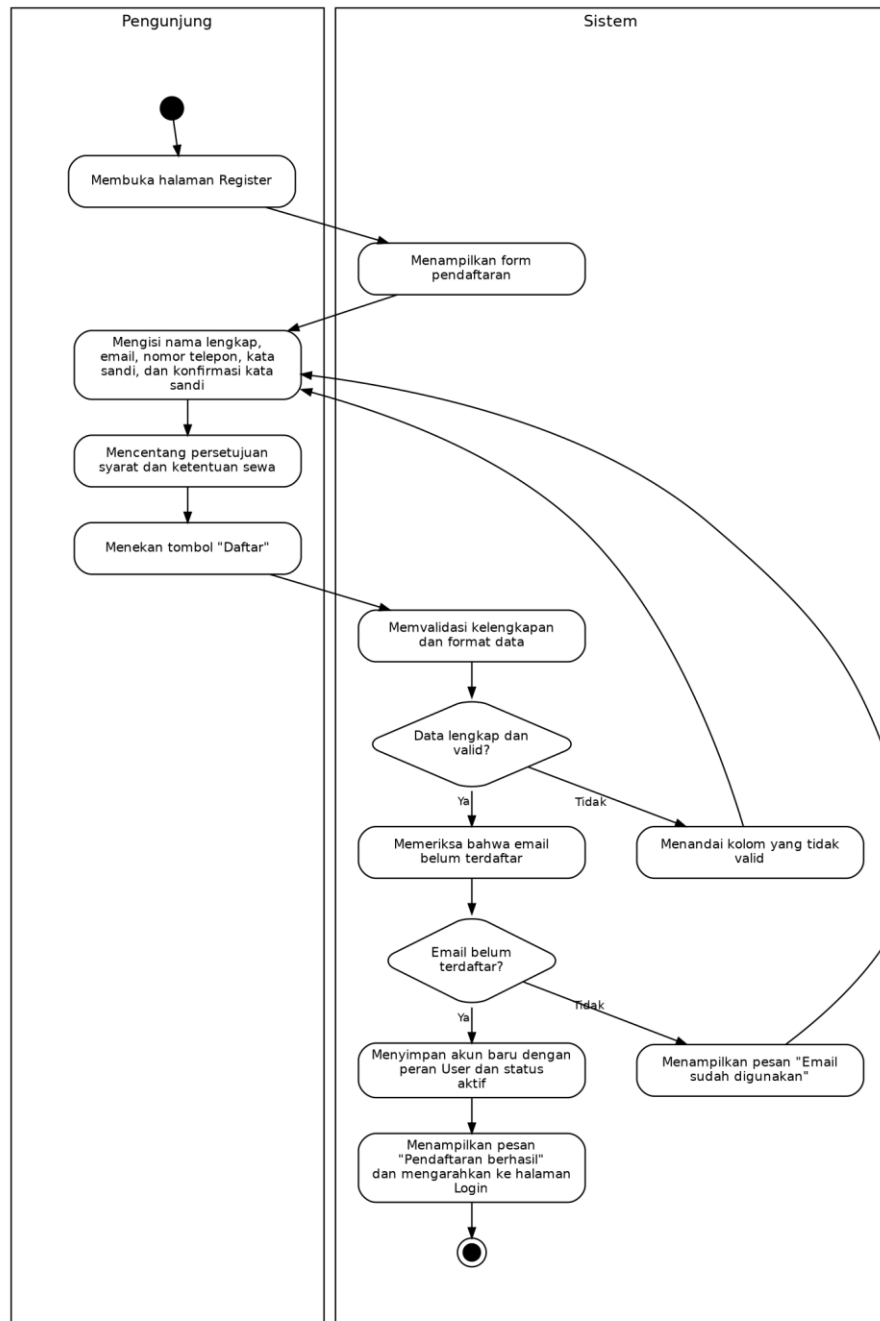
Gambar 3.4 Activity Diagram UC-02 Pendaftaran Akun
