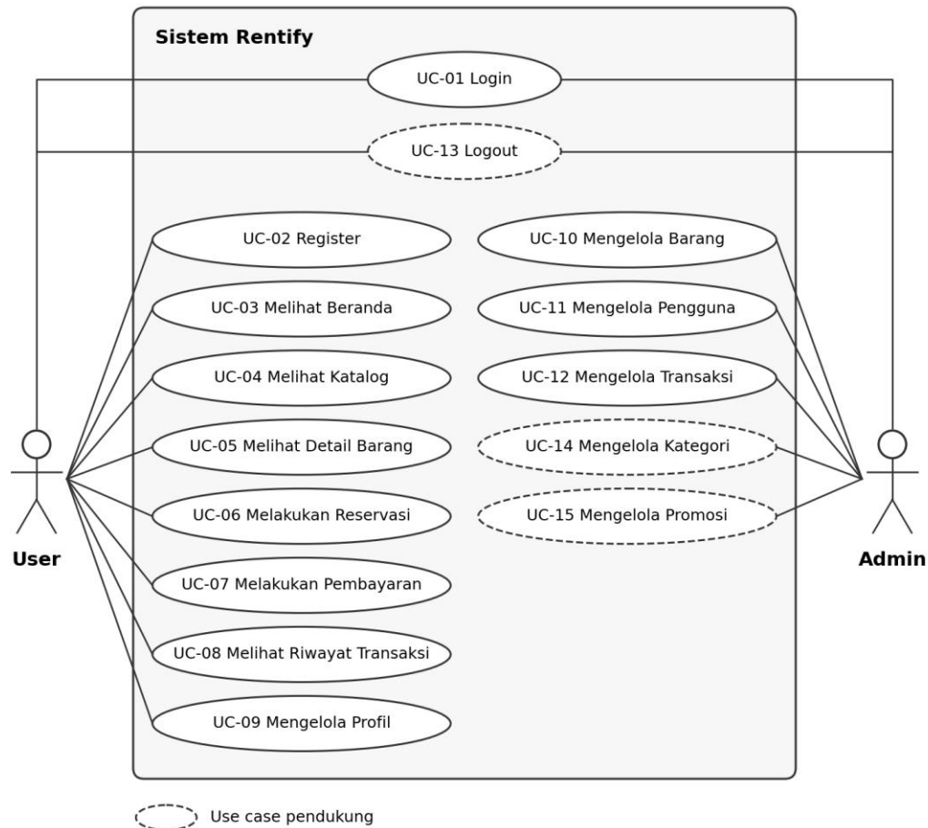
Gambar 3.1 Usecase Diagram Rentify
