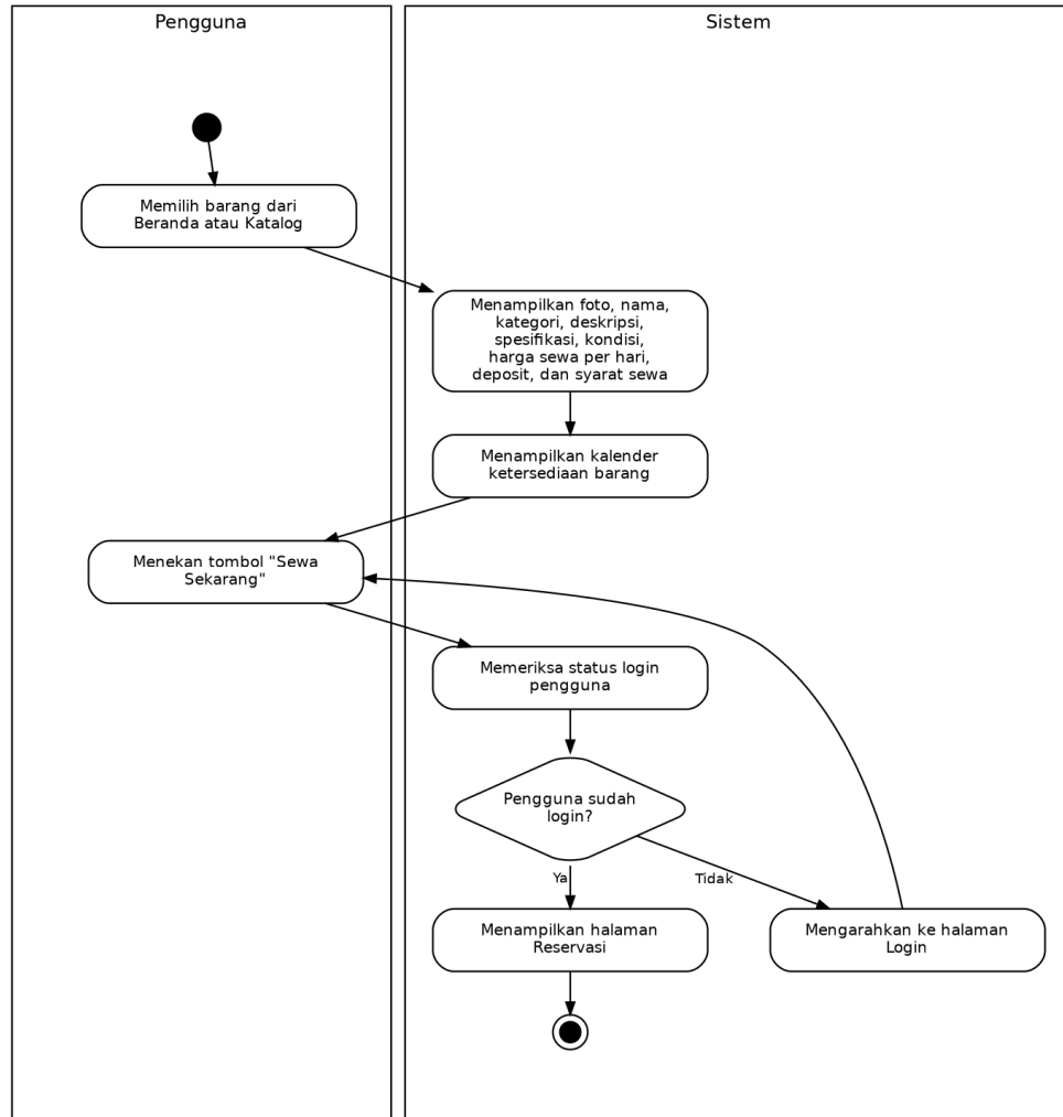
Gambar 3.7 Activity Diagram UC-05 Melihat Detail Barang
