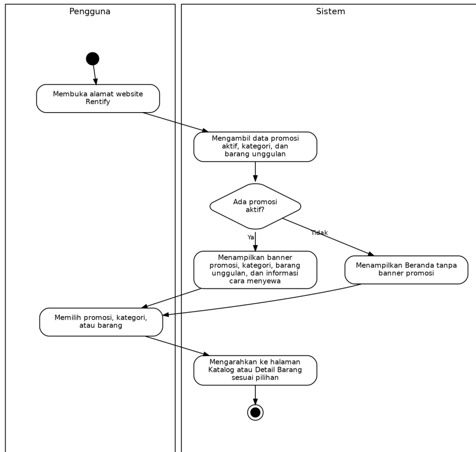
Gambar 3.5 Activity Diagram UC-03 Melihat Beranda
