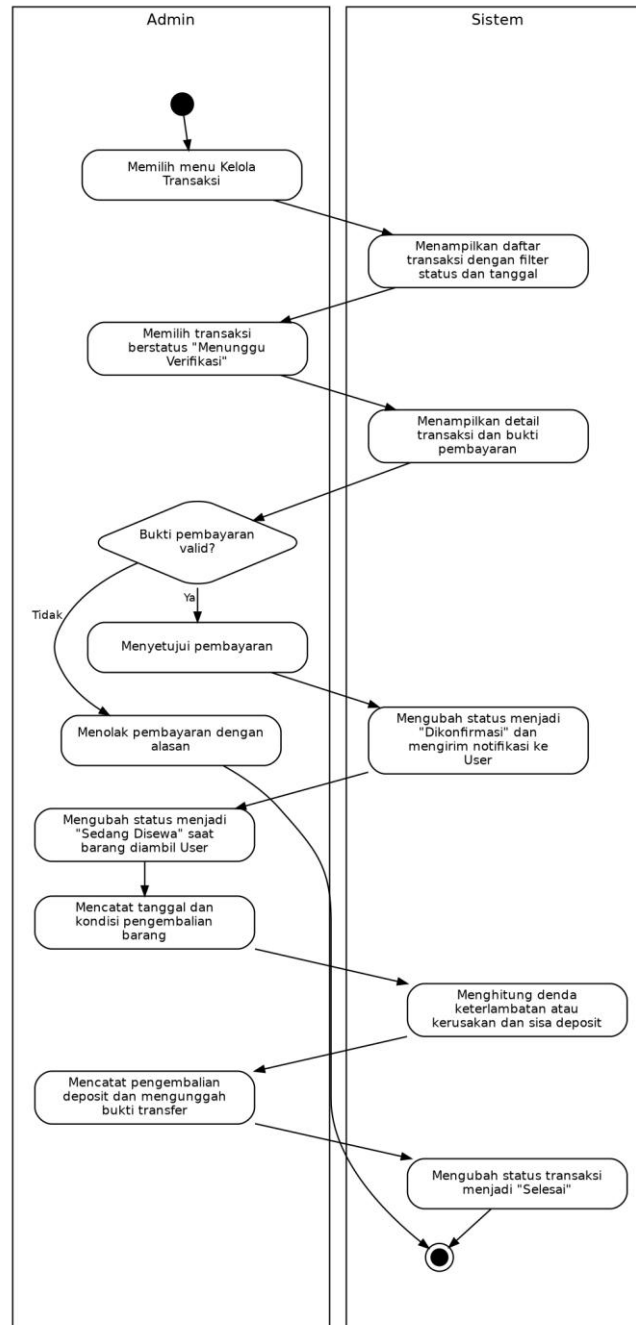
Gambar 3.14 Activity Diagram UC-12 Mengelola Transaksi
