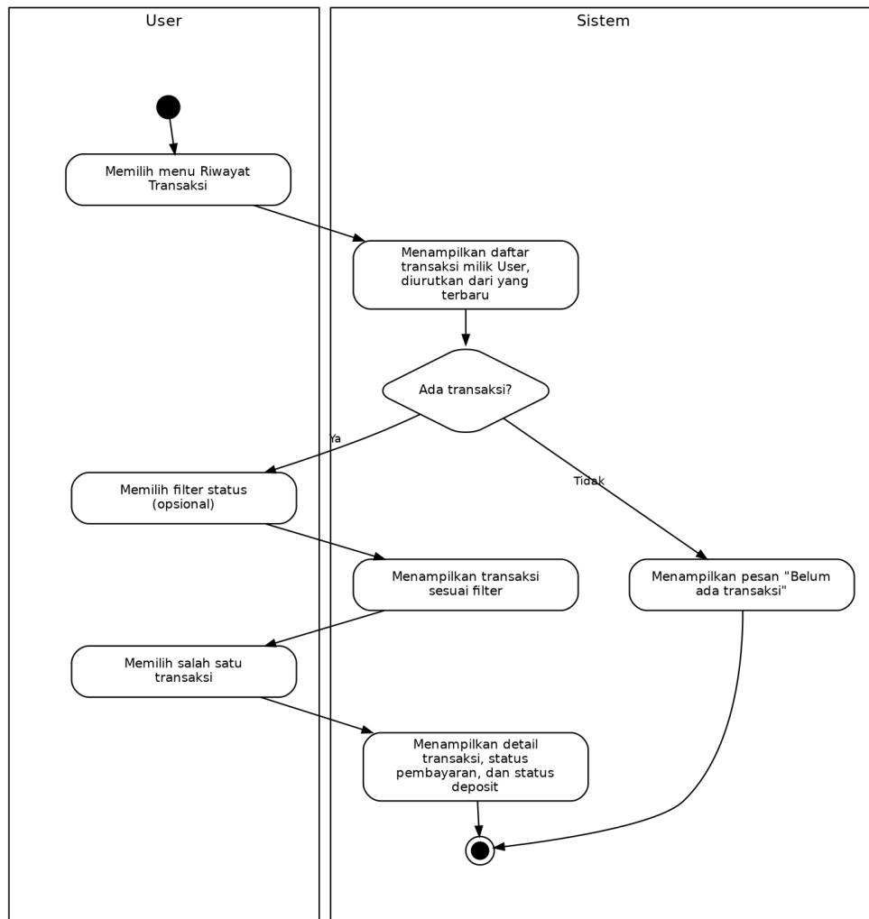
Gambar 3.10 Activity Diagram UC-08 Melihat Riwayat Transaksi
