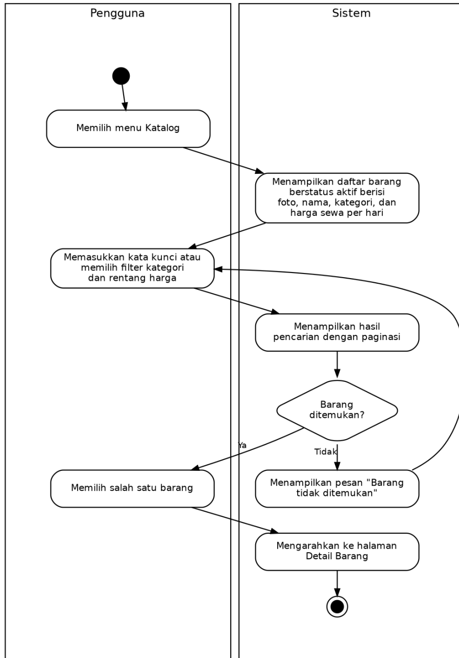
Gambar 3.6 Activity Diagram UC-04 Melihat Katalog
