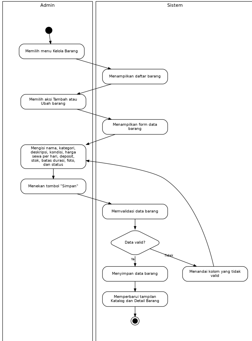
Gambar 3.12 Activity Diagram UC-10 Mengelola Barang
