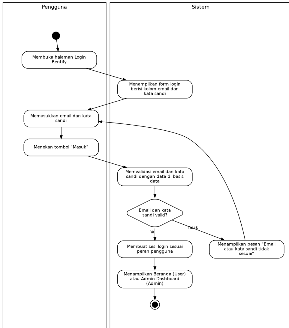
Gambar 3.3 Activity Diagram UC-01 Masuk Akun
