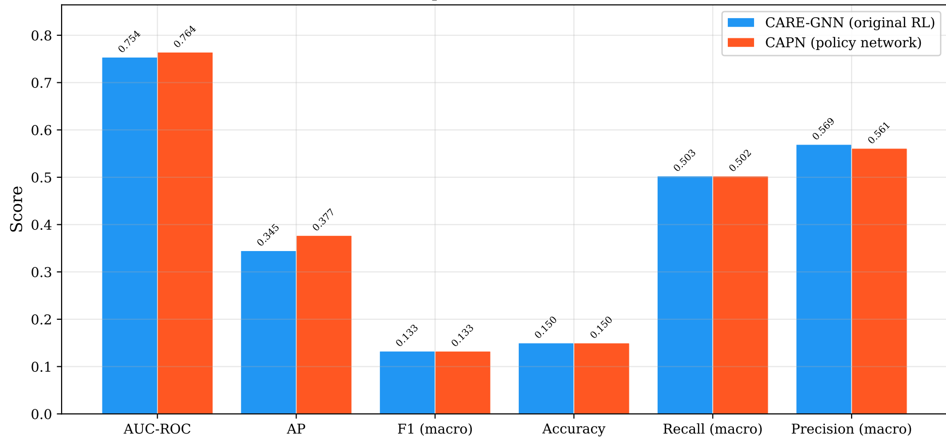
Capn — GNN Metrics
