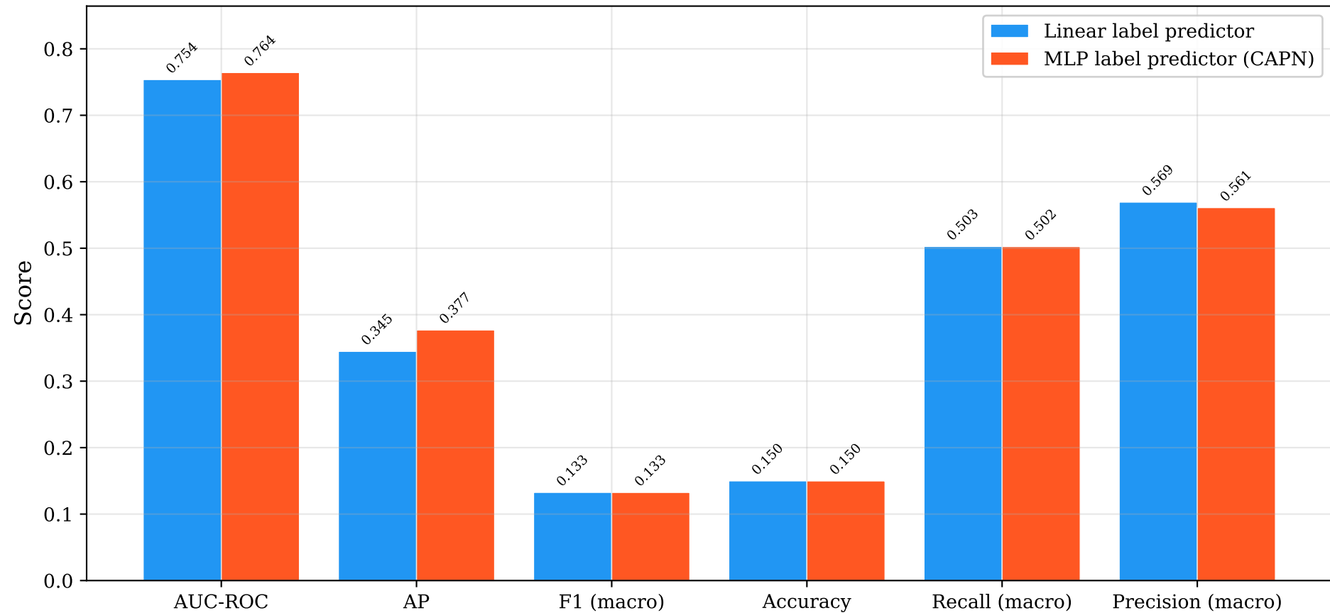
Capn Label — GNN Metrics
