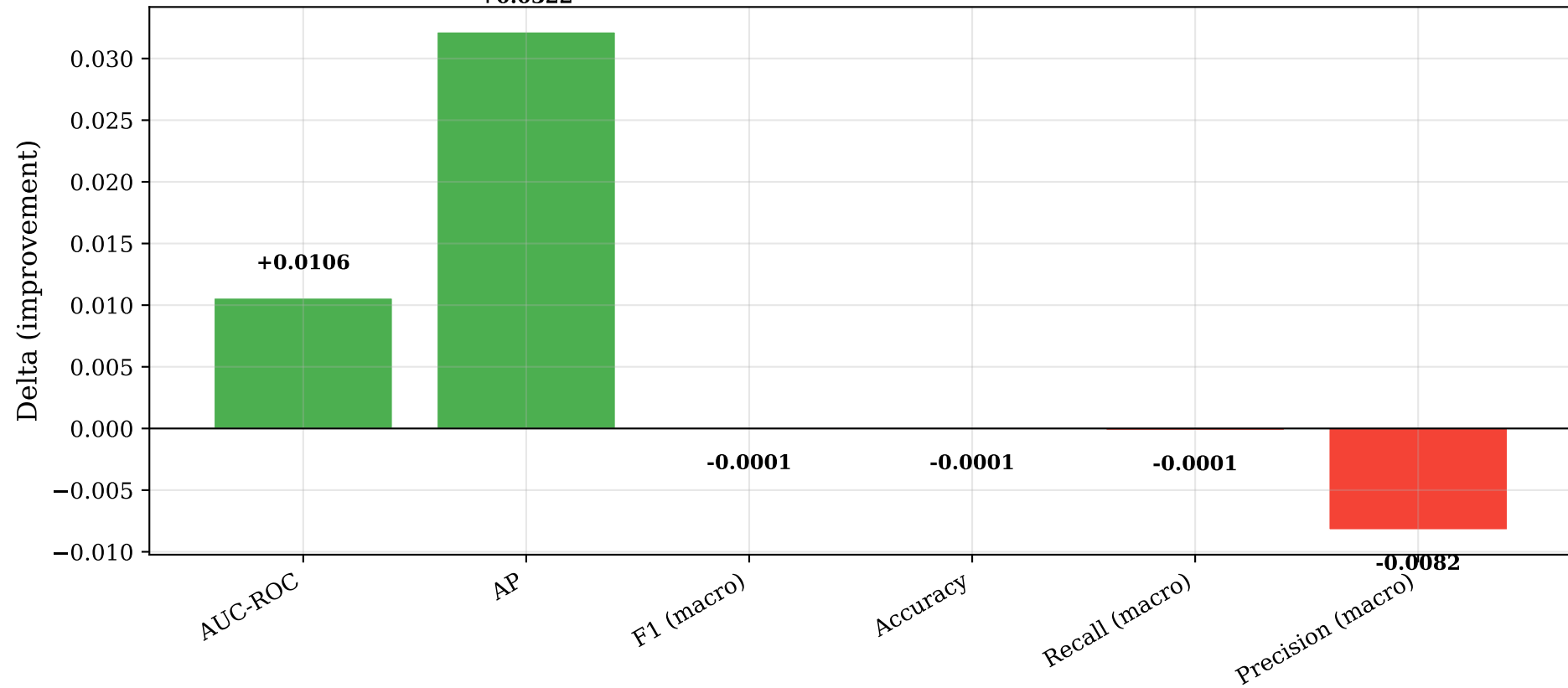
Improvement: MLP label predictor (CAPN) (MLP label predictor (CAPN) vs Linear label predictor)
