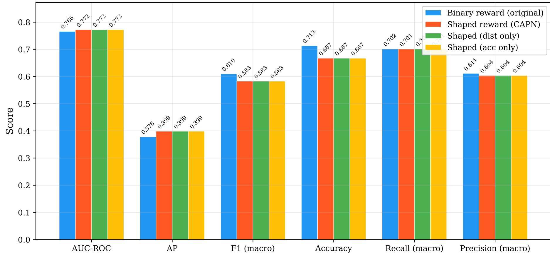
Capn Reward — GNN Metrics
