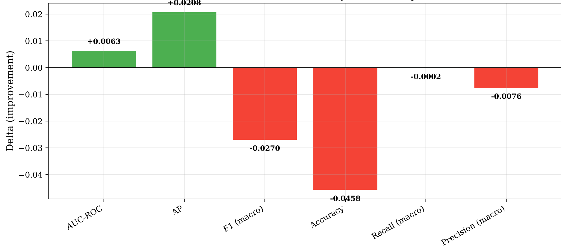
Improvement: Shaped reward (CAPN) (Shaped reward (CAPN) vs Binary reward (original))
