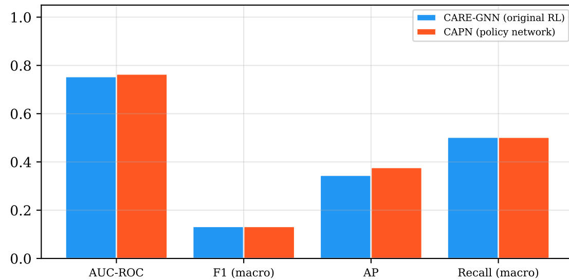
Capn
