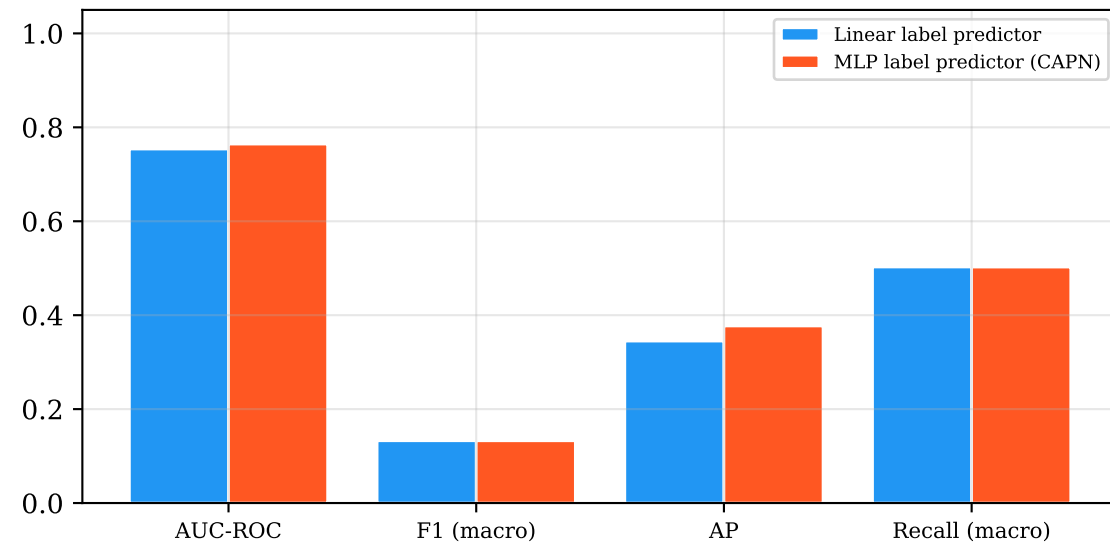
Capn Label
