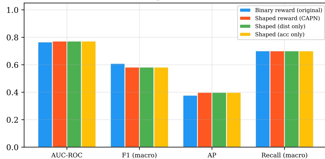
Capn Reward
