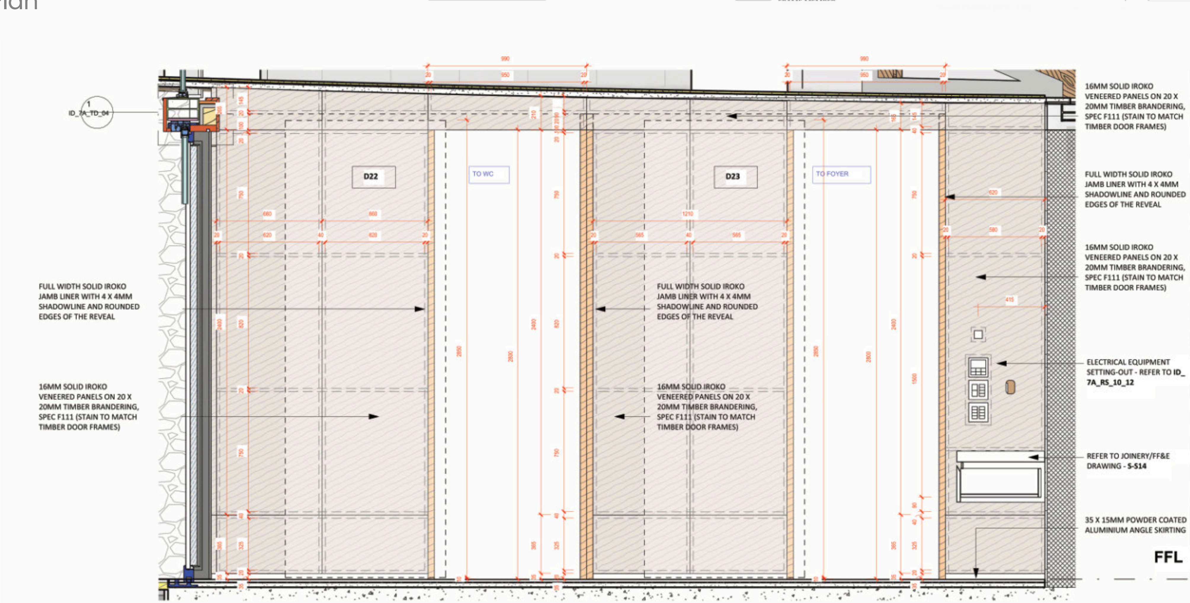
Front Elevation [without doors] NTS
