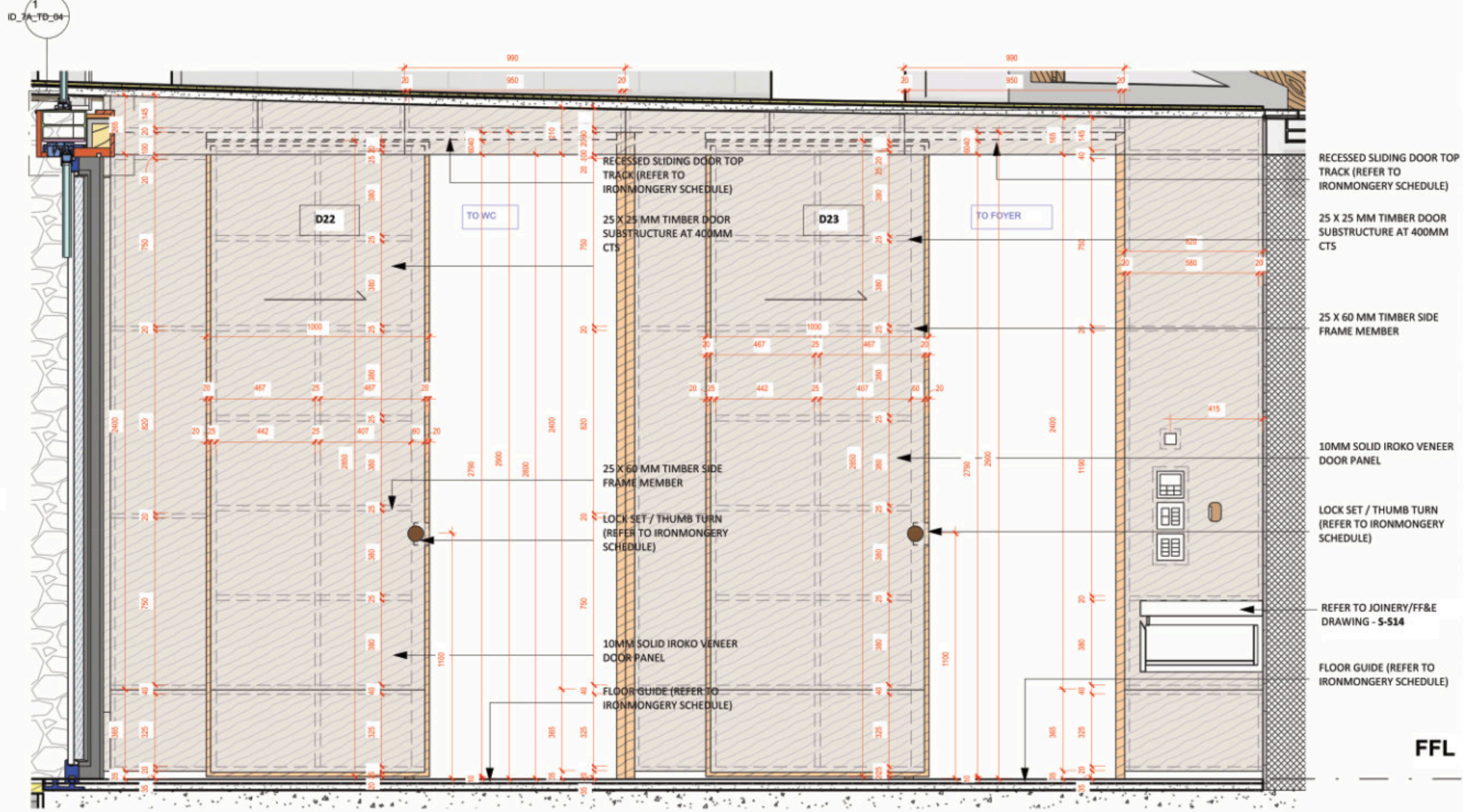
Front Elevation [with doors] NTS
